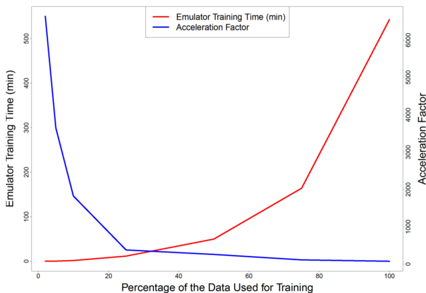
Figure 6. Effect of reducing the training dataset size on emulator training time (how long it takes to train the emulator) and acceleration factor (how many times is the emulator faster than the simulator).
