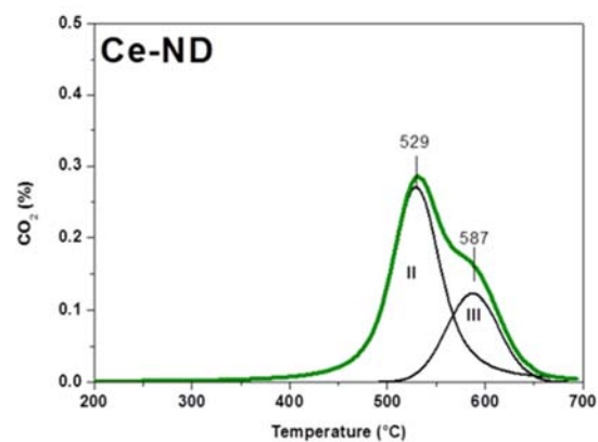
Classical ceria
