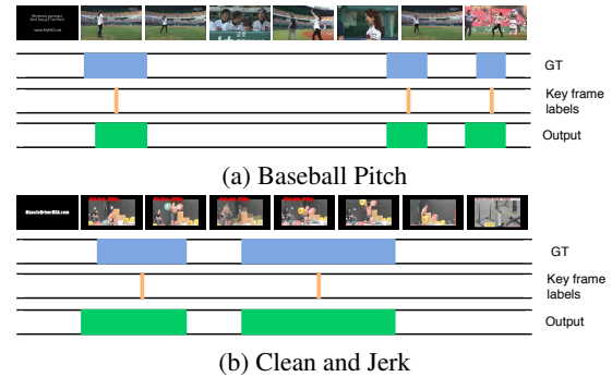
Fig. 1. Our proposed method. A single frame is labeled for each action instance. The detected results are shown for THUMOS'14 dataset. Using a single frame, the PU learning network is able to detect action boundaries with low error.
