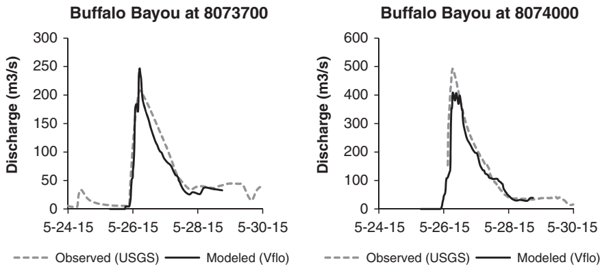
FIGURE 4 Stream flow comparisons for the Memorial Day 2015 Storm in Buffalo Bayou
