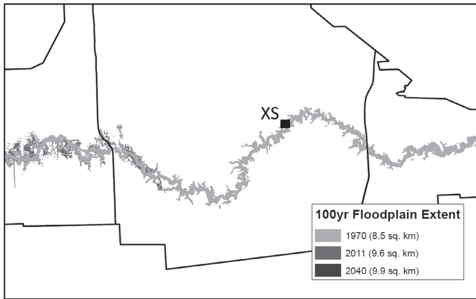
FIGURE 10 100-year floodplain with selected cross-sectional (XS) view at Buffalo Bayou
