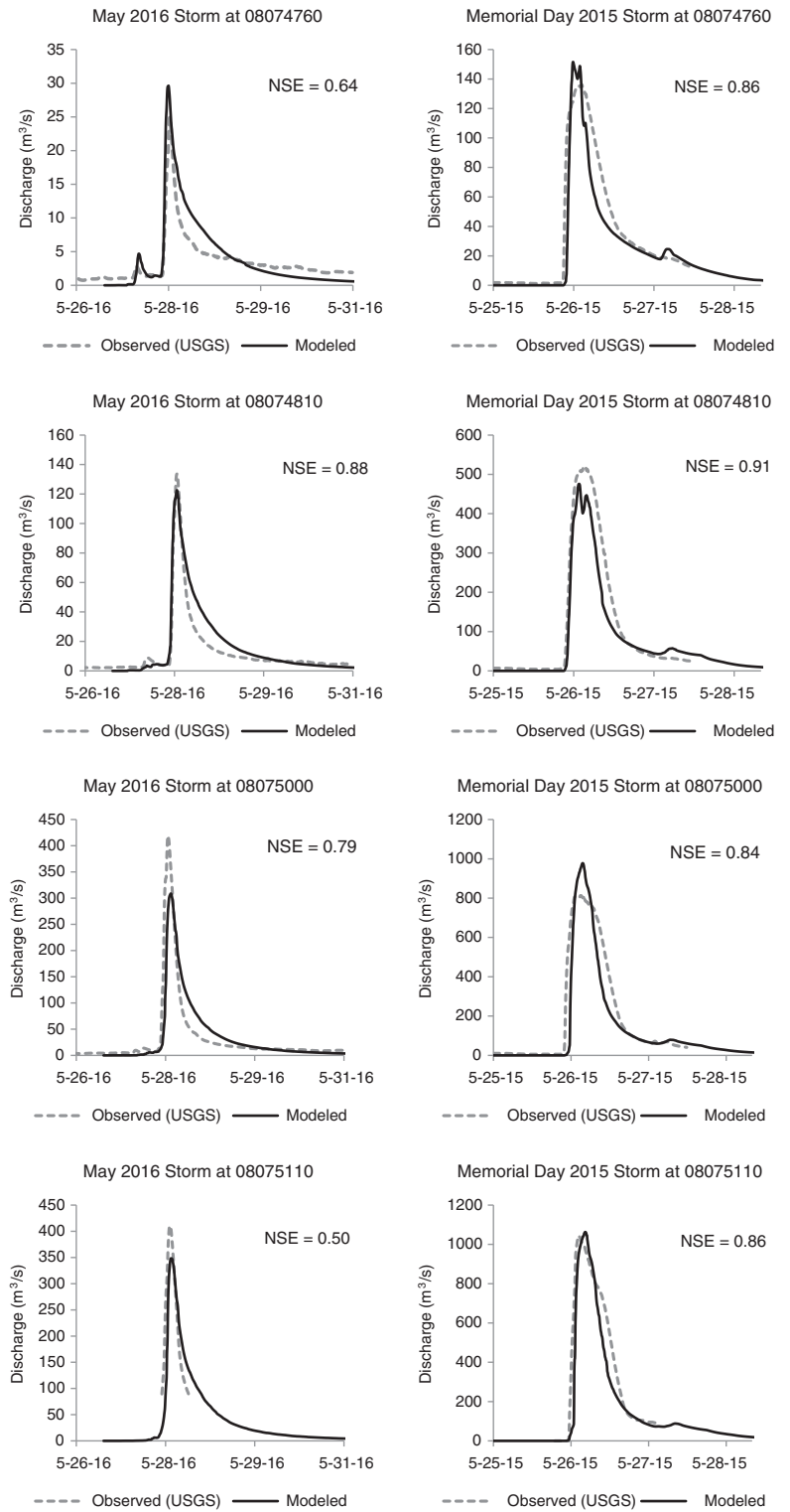
FIGURE B2 Stream flow comparisons in Brays Bayou
