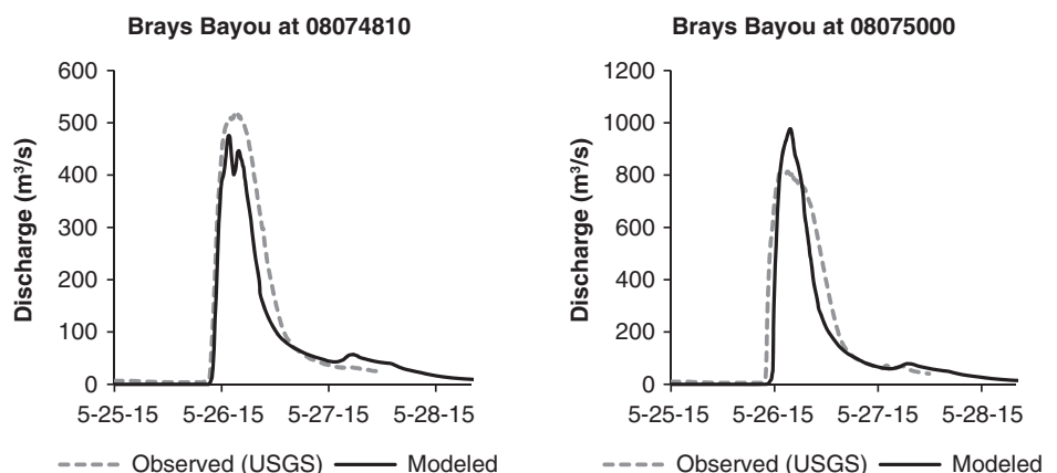
FIGURE 3 Stream flow comparisons for the Memorial Day 2015 Storm in Brays Bayou
