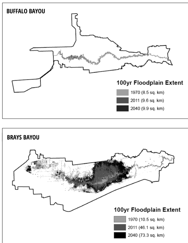
FIGURE 8 Modeled floodplains for Buffalo Bayou (unchannelized) and Brays Bayou (channelized) under three LULC scenarios
