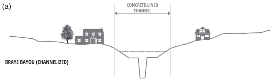
FIGURE 2 (a) Brays Bayou riverine management (channelized) schematic (Photo: Brays Bayou at Buffalo Speedway). (b) Buffalo Bayou riverine management (unchannelized) schematic (Photo: Buffalo Bayou near Waugh Dr.)
