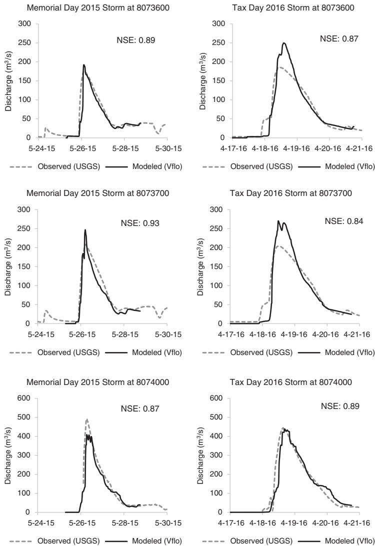
FIGURE B1 Stream flow comparisons in Buffalo Bayou
