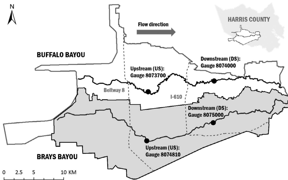
FIGURE 1 Brays Bayou and Buffalo Bayou watersheds, with watch point (gauge) location
