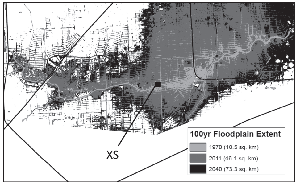
FIGURE 9 100-year floodplain with selected cross-sectional (XS) view at Brays Bayou
