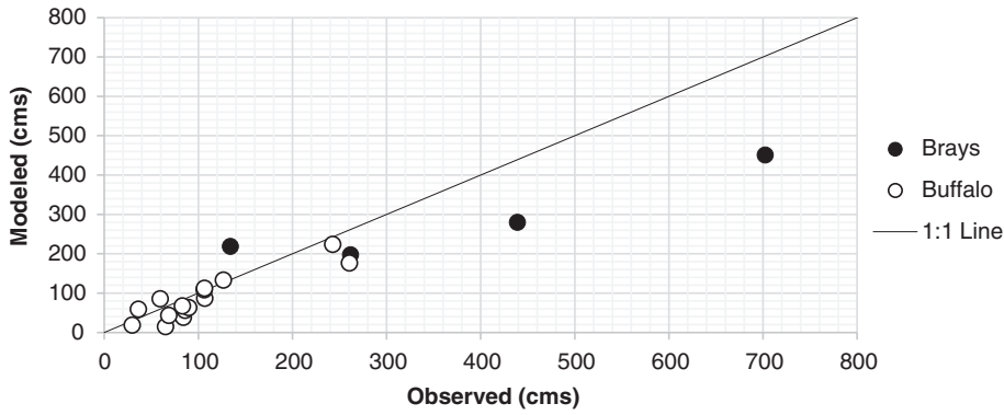
FIGURE A1 Model validation for the 1970s (historical) condition. Comparison between peak modeled and observed flows during five flood events (1967–1973) shown for gauges in Brays Bayou (solid) and Buffalo Bayou (open)
