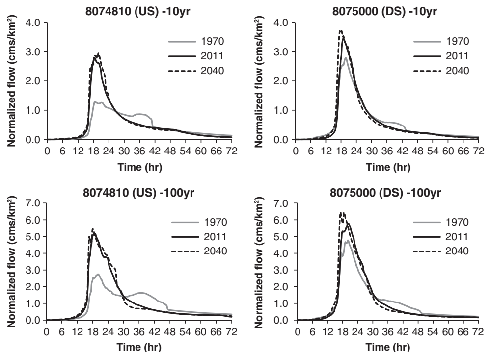
FIGURE 6 Modeled normalized streamflow (cms/km 2 ) for Brays Bayou under three LULC scenarios (US drainage area: 120.6 km 2 , DS drainage area: 219.5 km 2 )
