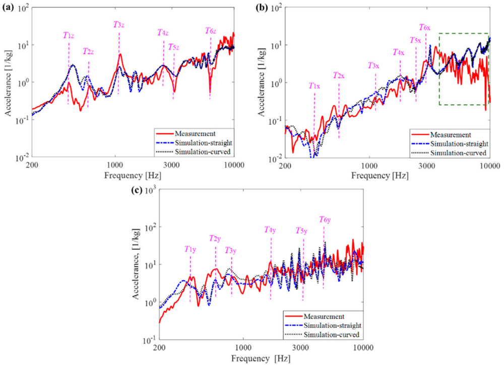
Figure 5. Comparison between simulated and measured track accelerances in the (a) vertical, (b) longitudinal, and (c) lateral directions. The dashed pink lines and corresponding notations ( T_{1x} , T_{1y} , T_{1z} ) indicate the characteristic frequencies of the track in three directions. The green dashed box in (b) marks the unreliable frequency range of the longitudinal hammer test using the self-made clamp.
