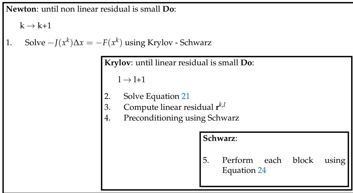
Figure 2. Newton–Krylov–Schwarz algorithm.
