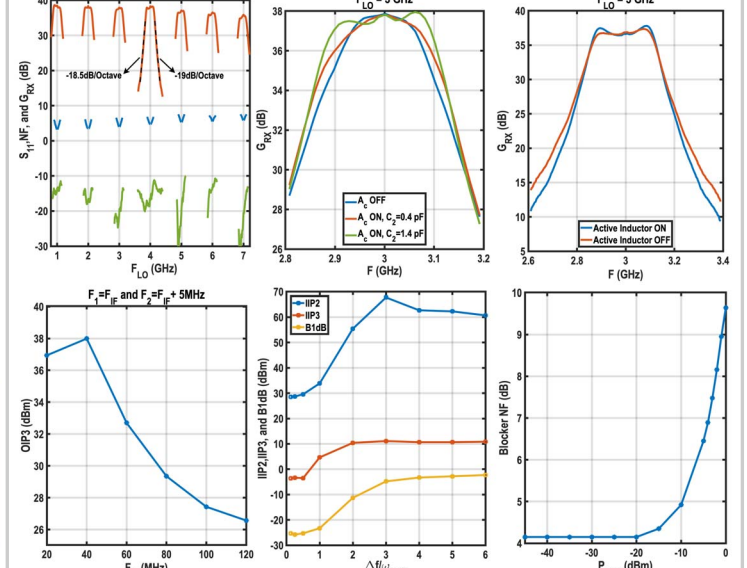
Figure 19.1.4: Small- and large-signal measurement results.
