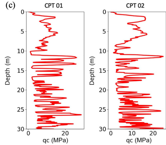
Figure 2 | (a) Location of the site and (b) the geometry of the reflection line. In (b), the red circles represent active sources, the blue circles represent receivers and the orange stars represent the locations of two cone penetration tests (CPTs). (c) Cone-tip resistance ( q_c ) was measured at the two CPT locations.
