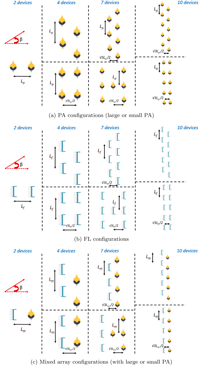
Fig. 3. Array configurations considered in this study: (a) PA arrays, (b) FL arrays, and (c) mixed arrays.
