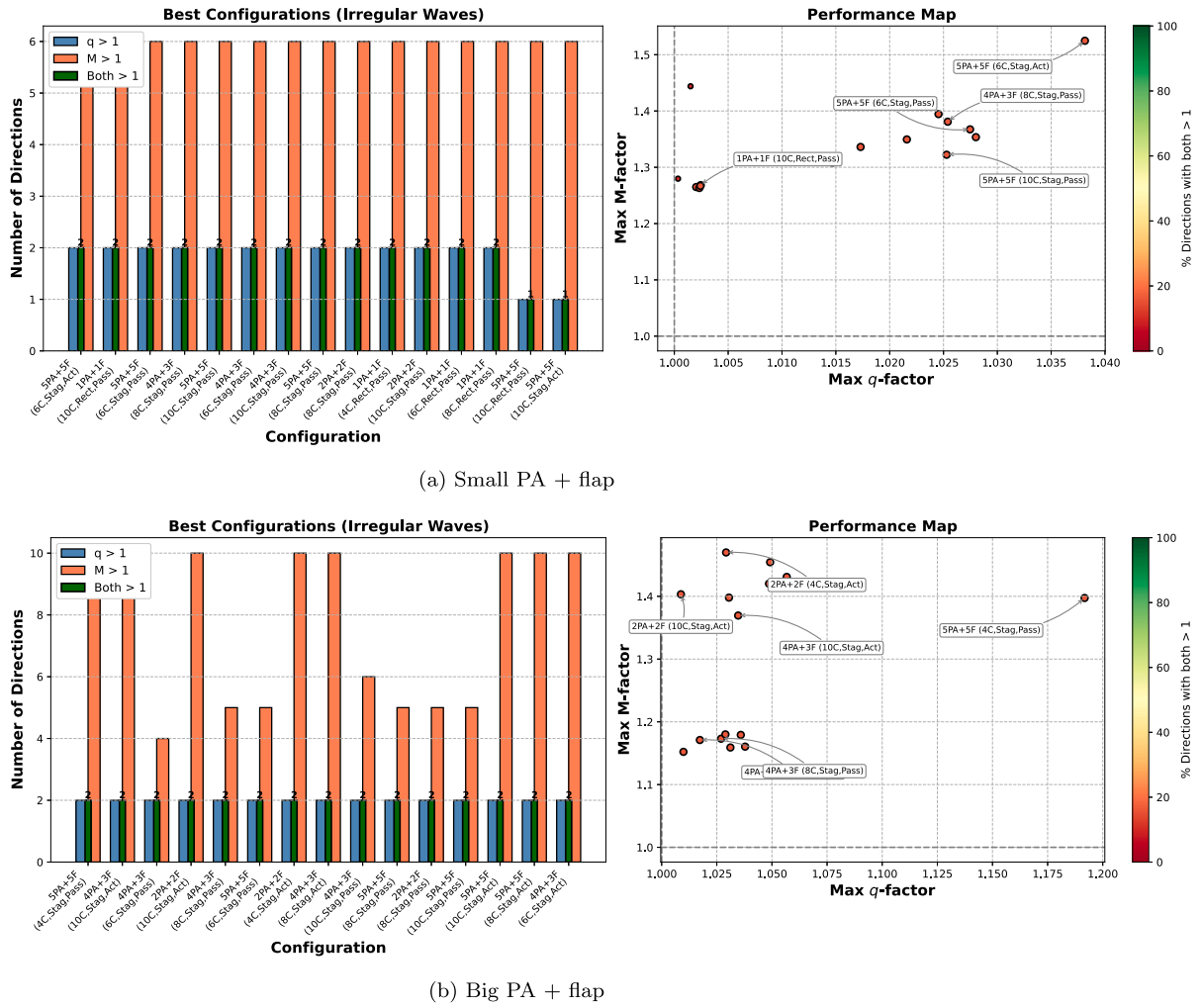
Fig. 11. Best-performing mixed array configurations under irregular wave conditions.
