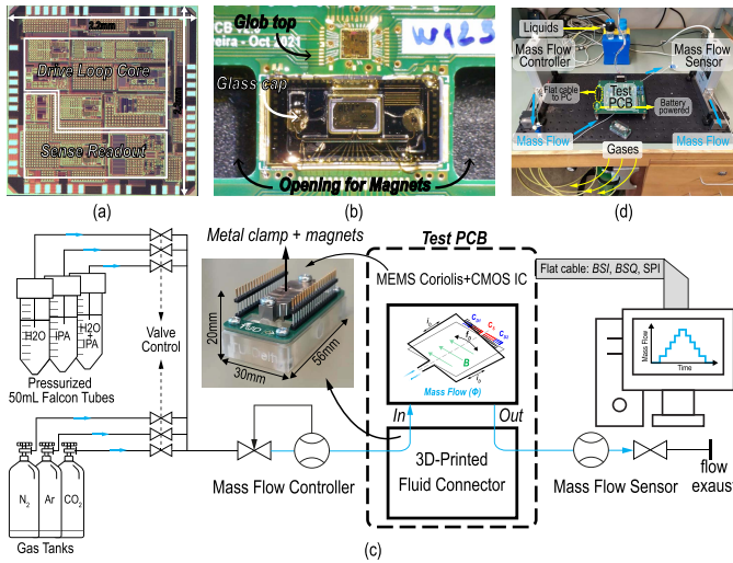
Fig. 11. (a) Micrograph of the fabricated 0.18- \mu m CMOS sensor interface. (b) Chip-on-board co-integration with the SCT-fabricated MEMS Coriolis mass flow sensor. (c) Mass flow measurement setup illustration, 3D printed fluid connector close-up, and (d) photograph of the actual setup.
