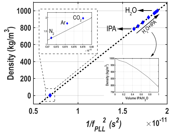
Fig. 18. Measured density to resonance frequency relationship.
