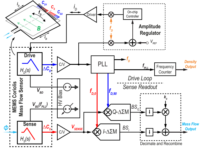
Fig. 4. System overview of the MEMS Coriolis ΦDC.
