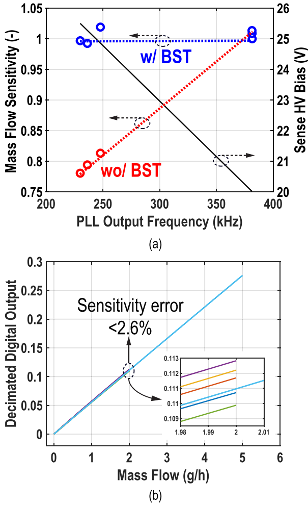
Fig. 13. (a) Normalized mass flow sensitivity versus resonance frequency. (b) Mass flow response after BST.
