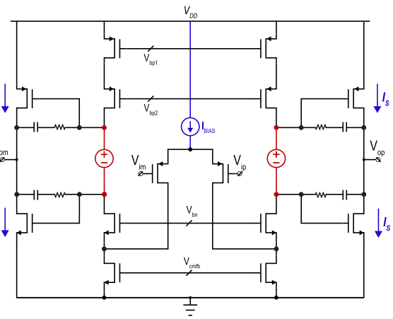
Fig. 6. Schematic of the two-stage op-amp used to implement the driver.
