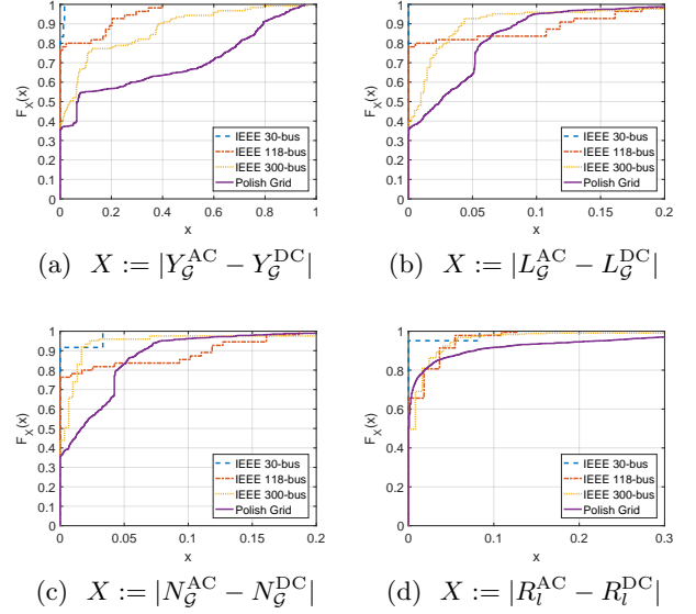
Figure 4: The CDFs of the differences between the metrics after cascading failures initiated by single line failures under the AC and DC models for all the test networks.
