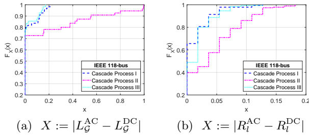
Figure 6: The CDFs of the differences between the metrics after cascades under the AC and DC models for the three cascade processes initiated by single line failures in the IEEE 118-bus network and Polish grid.
