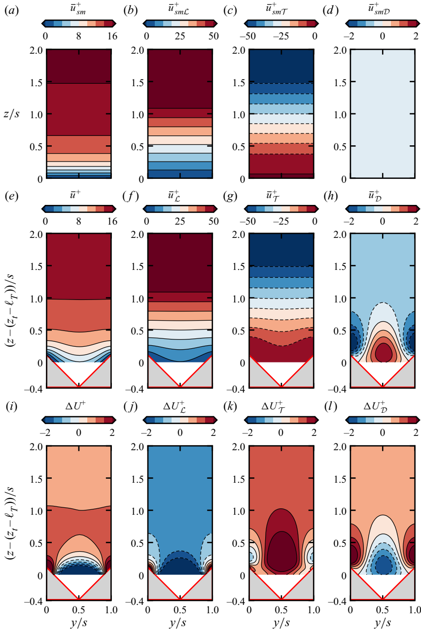
Figure 15. (a) Mean streamwise velocity over the smooth wall \bar{u}_{sm}^+ = \bar{u}_{smL}^+ + \bar{u}_{smT}^+ + \bar{u}_{smD}^+ and its FIK contributions: (b) laminar \bar{u}_{smL}^+ , (c) turbulent \bar{u}_{smT}^+ , (d) dispersive \bar{u}_{smD}^+ . (e) Mean streamwise velocity over the riblet case TI950 \bar{u}^+ = \bar{u}_L^+ + \bar{u}_T^+ + \bar{u}_D^+ and its FIK contributions: (f) laminar \bar{u}_L^+ , (g) turbulent \bar{u}_T^+ , (h) dispersive \bar{u}_D^+ . (i) Hama roughness function and its FIK contributions: (j) laminar \Delta U_L^+ = \bar{u}_{smL}^+ - \bar{u}_L^+ , (k) turbulent \Delta U_T^+ = \bar{u}_{smT}^+ - \bar{u}_T^+ , (l) dispersive \Delta U_D^+ = \bar{u}_{smD}^+ - \bar{u}_D^+ .
