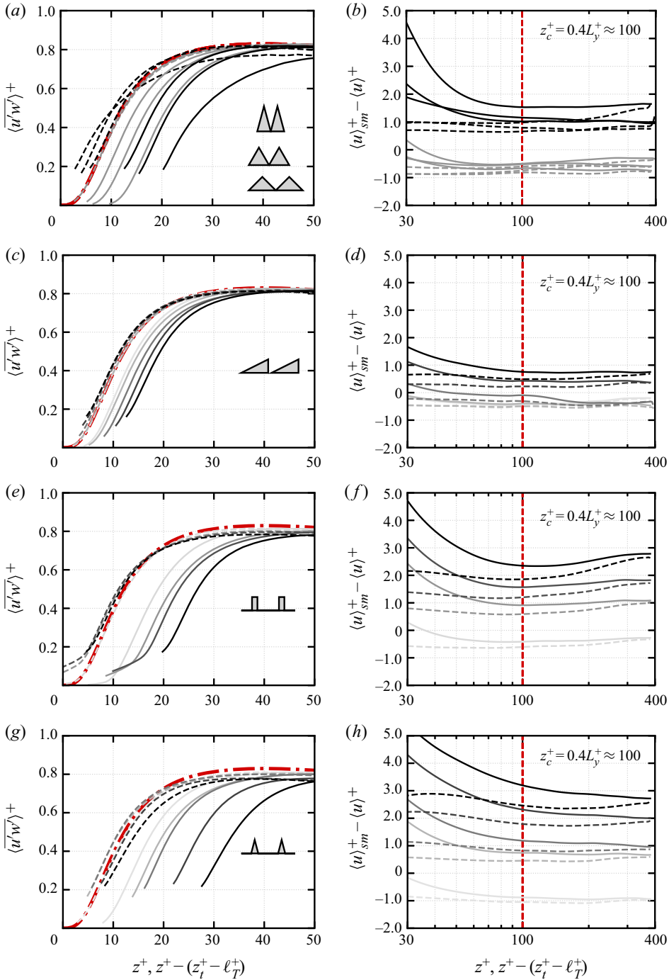
Figure 4. Turbulent stress \overline{u'w'}^+ (a,c,e,g) and Hama roughness function \langle u \rangle_{sm}^+ - \langle u \rangle^+ (b,d,f,h), for triangular (a,b), asymmetric triangular (c,d), blade (e,f) and trapezoidal riblets (g,h). Profiles are reported with respect to the constant volume origin at z = 0 (black solid line) and with respect to the origin of the turbulent stress at z = z_t - \ell_T (black dashed line). Colour from light to dark indicates increasing riblets spacing s^+ (table 1). The smooth wall minimal-channel turbulent stress (red dashed dot line thick) is also reported in (a,c,e,g). Profiles are shown from above the crest. z_c^+ = 0.4L_y^+ \approx 100 (table 1), represented by the red dashed line, is the critical height at which \Delta U^+ is measured. Here, z_t indicates the location of the crest and \ell_T the location of the virtual origin, measured downward from the crest.
