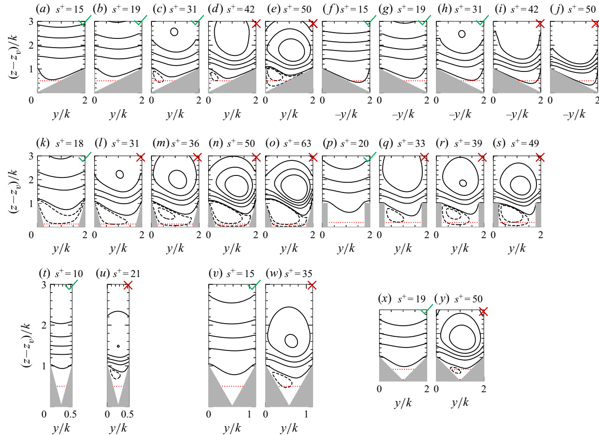
917 A55-21 Figure 12. Streamfunction of the mean conditional cross-flow, conditioned to the direction of mean spanwise flow at the riblet crest. The mean flow just above the groove is from left to right for all cases, apart from asymmetric riblets ( f-j ) which show the flow from right to left. To ease comparison these plots are mirrored. The lines are for constant values of the conditional streamfunction in the cross-section \psi_r^+ = (0.2, 5.2, 10.2, 15.2, 20.2) \times 10^{-3} (solid lines) for counter-clockwise rotation and \psi_r^+ = (-6, -1) \times 10^{-4} (dashed lines) for clockwise rotation. The red dotted line indicates the riblet mean height. The green tick (✓) indicates drag-decreasing cases, the red cross (✗) drag-increasing cases.
