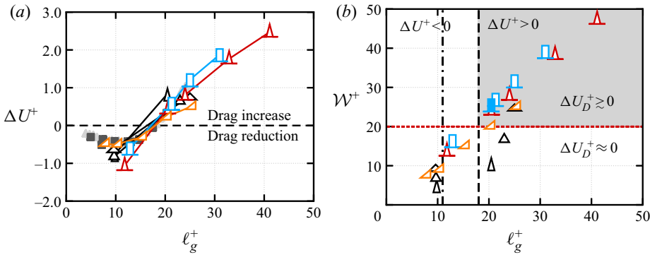
Figure 18. (a) Mean velocity shift \Delta U^+ as a function of \ell_g^+ and (b) viscous-scaled groove width at the riblet mean height W^+ as a function of the viscous-scaled square root of the groove area \ell_g^+ for all flow cases. The vertical black dashed line indicates \ell_g^+ = 18 , the vertical black dash-dotted line \ell_g^+ = 11 and the horizontal red line W^+ = 20 . The shaded region indicates the drag-increasing regime in which dispersion contribute more than turbulence to the breakdown of drag reduction \Delta U_D^+ > \Delta U_T^+ . The filled symbol in (b) refers to the s/t = 4 blade riblets data of García-Mayoral & Jiménez (2011).
