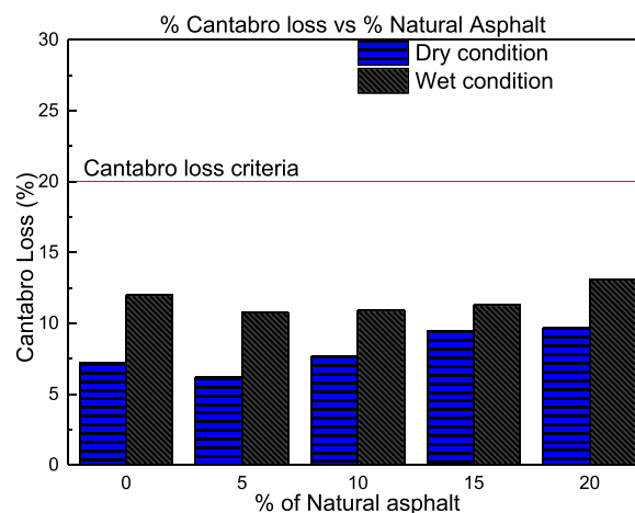
Fig. 10. Cantabro loss % of asphalt-modified Natural bitumen.
