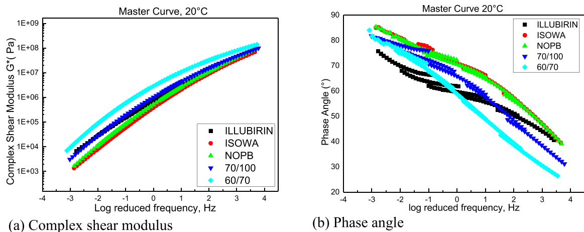
Fig. 4. (a) Complex shear modulus and Phase angle for Natural and petroleum bitumen.
