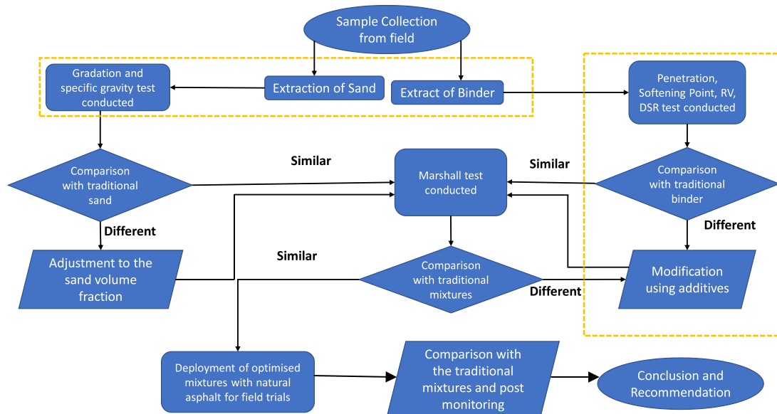
Fig. 1. Optimization of Natural bitumen for road construction. Note: Traditional mixtures: Typical dense asphalt mixtures of different aggregate sizes and 60/70 bitumen. Traditional Binder: The typical 60/70 penetration grade bitumen used in Nigeria for road construction.
