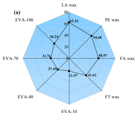
Fig. 16. Binding energy values (kJ/mol) of (a) Asphaltenes and WWM additives and EVA and (b) EVA and WWM additives.
