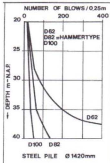
Figure 10: Results drivability of open steel tubular piles (Mourilon, 2015)
