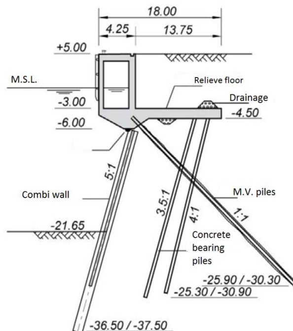
Figure 4: Cross section old quay to be demolished (Gijt, 2013)
