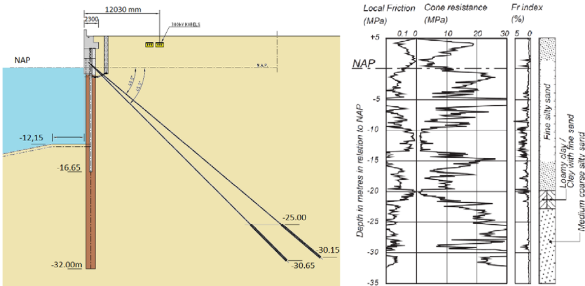
Figure 3: Cross section quay wall and typical CPT for Maasvlakte area
