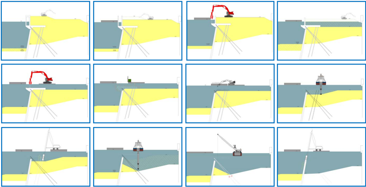
Figure 5: Demolition and excavation sequence.
