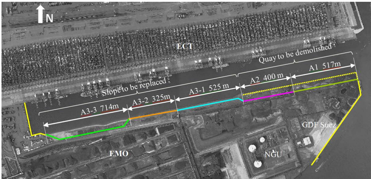
Figure 2: Aerial picture with in color the new basin shape & quay wall
