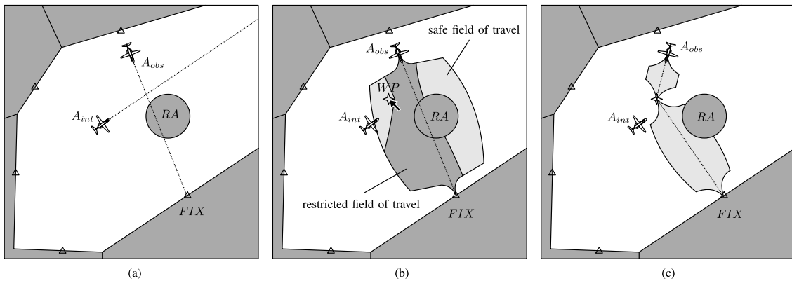
Fig. 2: TSR in an hypothetical traffic scenario. (a) Traffic scenario with two conflicting aircraft and a restricted airspace. (b) TSR and placement of an intermediate waypoint. (c) Resulting trajectory for the observed aircraft [4].
