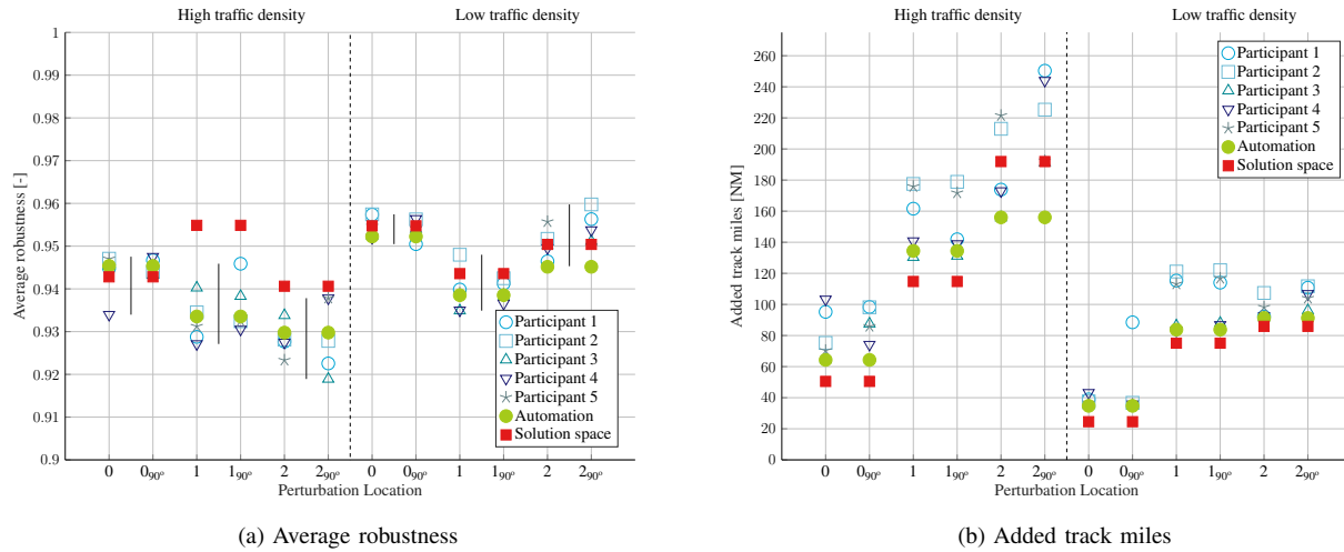
Fig. 8: Average sector robustness and added track miles per perturbation location and traffic density.
