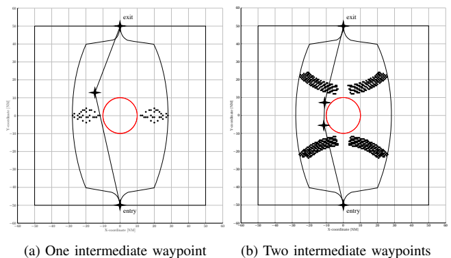
Fig. 3: Solution space for one and two additional waypoints. The points within the solution space shape represent the possible algorithm solutions, whereas the crosses and straight lines represent the human solutions.
