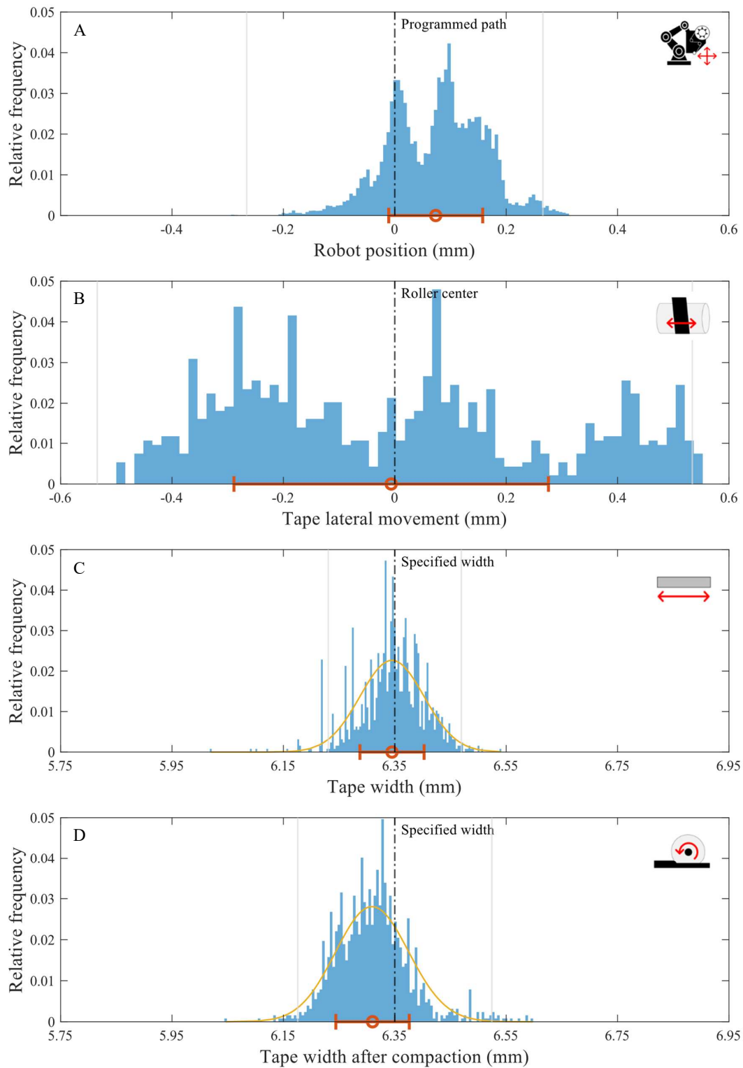
Figure 9: A, B, C, D (top to bottom) Measured manufacturing variations which cause gaps and overlaps. Note that the X and Y axes are equally scaled. Means and \pm 1\sigma values are annotated in orange. 99 th percentile deviation values are annotated by grey lines. Fits are annotated in yellow.
