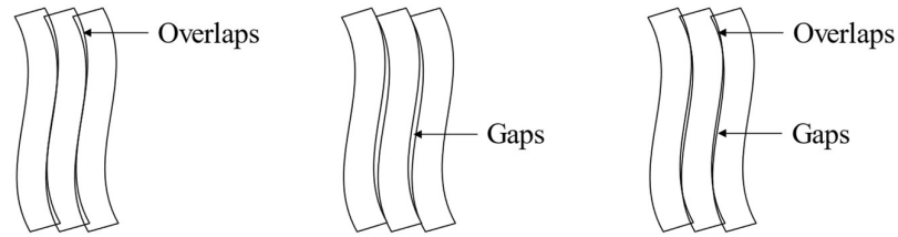
Figure 2: Gaps and overlaps due to shifting of tow path
