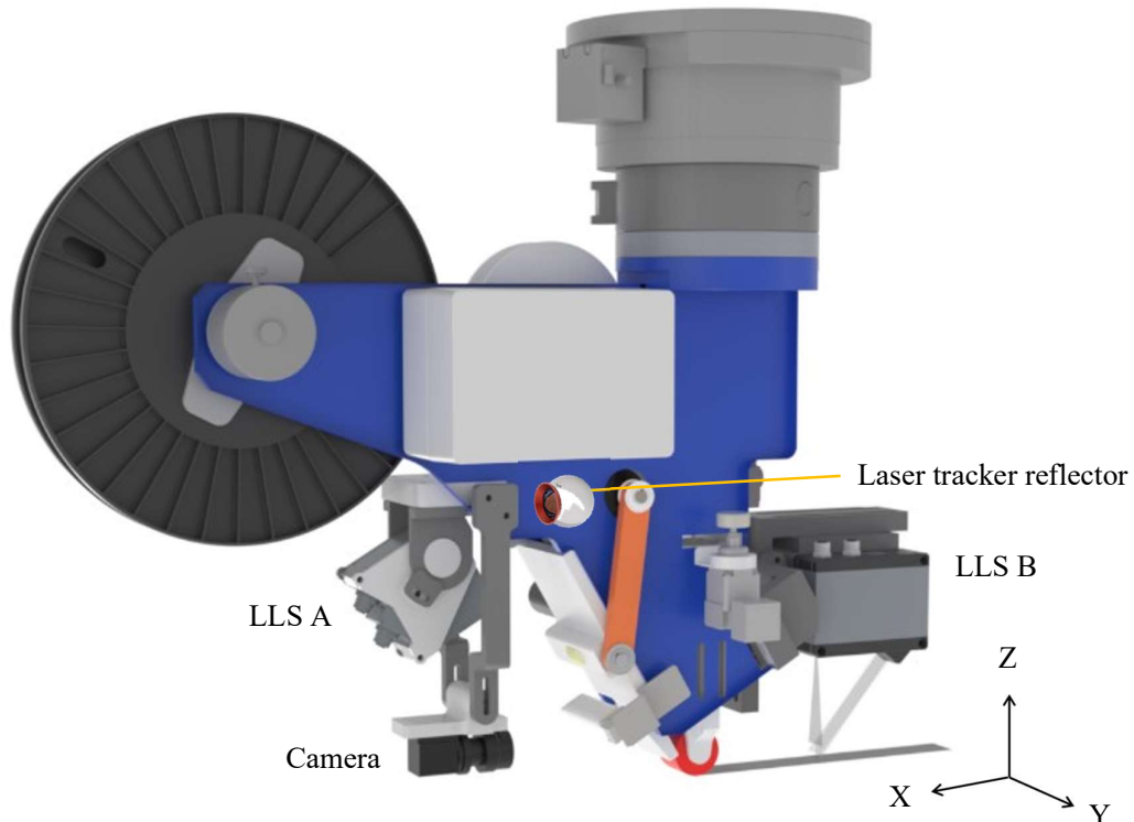
Figure 5: CAD model showing various sensors setup on the AFP head. Layup is in positive X direction.
