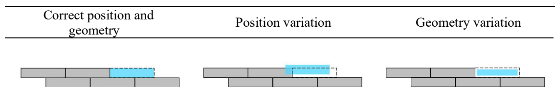
Figure 3: AFP tape layup cross section schematic – ideal tape placement (left), tape placement with position variation (middle), tape placement with geometry variation (right)
