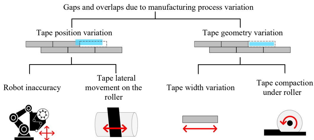
Figure 4: Breakdown of AFP manufacturing process variations which cause gap and overlap defects.
