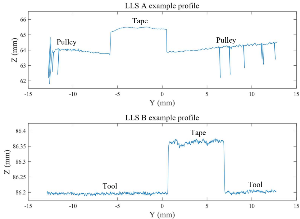
Figure 8: Example profiles measured by the two laser line scanners
