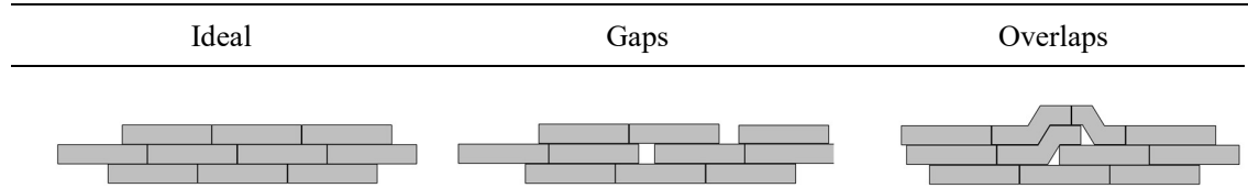
Figure 1: AFP tape layup cross section schematic – ideal AFP composite mesostructure with abutting tapes (left), gaps (middle) and overlaps (right).
