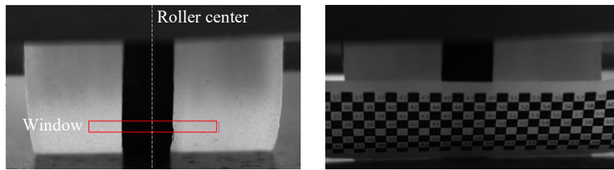
Figure 7: Example frame recorded by the camera. Annotations show the roller center line and the measurement window (Left). Reference image with a checkerboard scale (Right).
