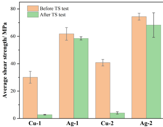
Fig. 19 – Average shear strength of the sintered joints before and after temperature shock.
