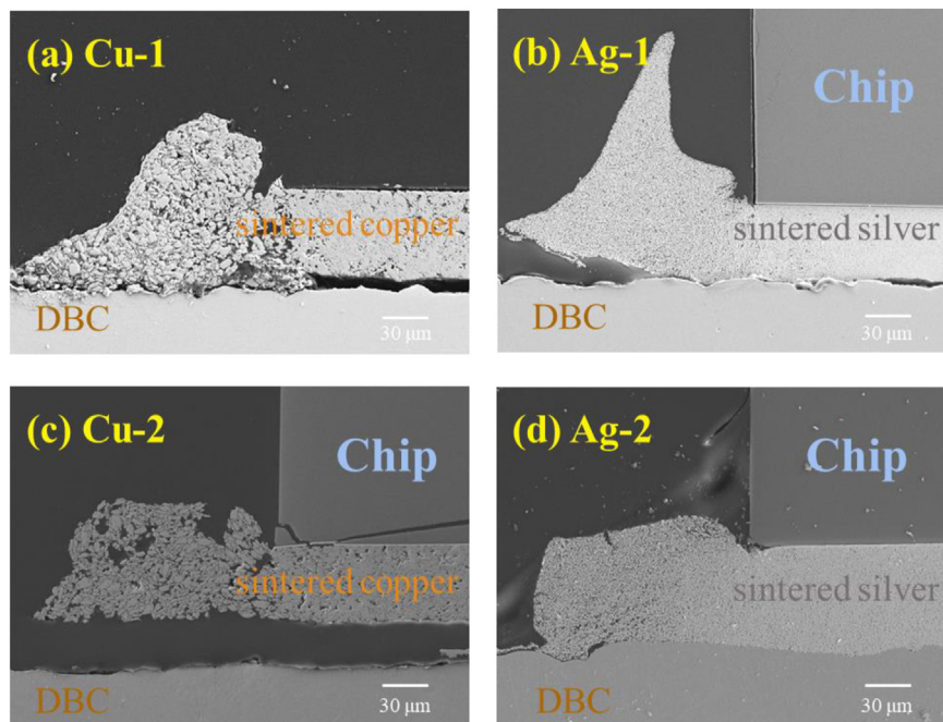
Fig. 20 – SEM photos of the joints after thermal shock (a)Cu-1; (b)Ag-1; (c)Cu-2; (d)Ag-2.
