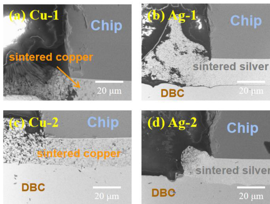
Fig. 9 – Cross section SEM photos of the joints after corrosion (a) Cu-1; (b) Ag-1; (c) Cu-2; (d) Ag-2.
