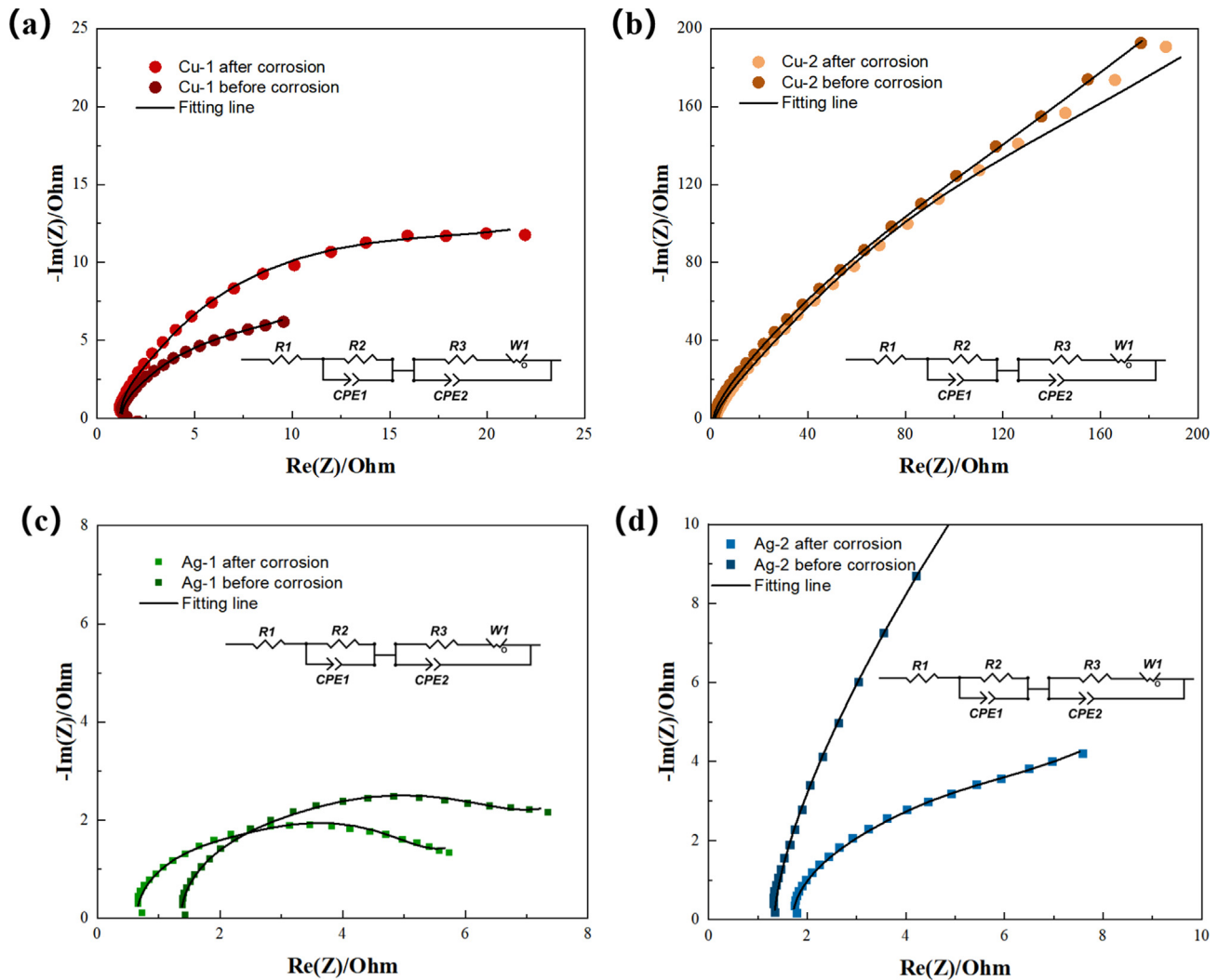
Fig. 15 – Initial EIS spectra of (a) Cu-1, (b) Cu-2, (c) Ag-1, and (d) Ag-2 sintered pastes before and after corrosion. An inset equivalent circuit of R_1(CPE_1R_2)(CPE_2(R_3W_1)) is used to simulate the resistances. Among them, R_1 is the ohmic resistance of the solution, R_2 and R_3 are the charge-transfer resistance of samples, CPE_1 and CPE_2 are the double-layer capacitance, and W_1 is the Warburg impedance.
