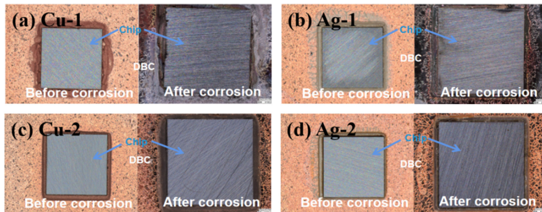
Fig. 5 – OM photos of the surface before and after corrosion (a) Cu-1; (b) Ag-1; (c) Cu-2; (d) Ag-2.
