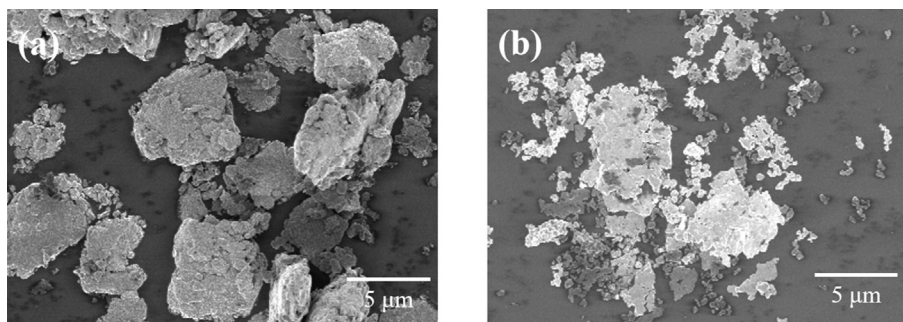
Fig. 2 – SEM photos of (a) Cu particles and (b) Ag particles.
