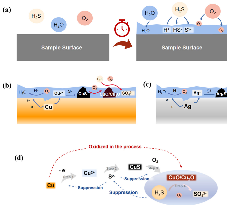
Fig. 18 – Schematic diagram of (a) changes in the surface of the sample after the corrosion; (b) corrosion mechanism of sintered copper surface; (c) corrosion mechanism of sintered silver surface; (d) the mechanism of copper oxide to further suppress copper corrosion.
