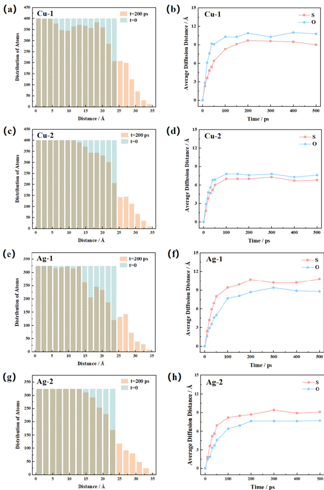
Fig. 17 – Initial and last distribution ( t = 200 ps) of Cu in models for (a)Cu-1 and (c)Cu-2. Initial and last distribution ( t = 200 ps) of Ag in models for (e)Ag-1 and (g)Ag-2. (b), (d), (f), and (h) Average diffusion distance of elements S and O.
