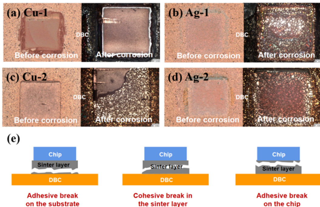
Fig. 8 – OM photos of the shear fractured surface before and after corrosion (a) Cu-1; (b) Ag-1; (c) Cu-2; (d) Ag-2. (e) Schematic diagram of the fracture modes.
