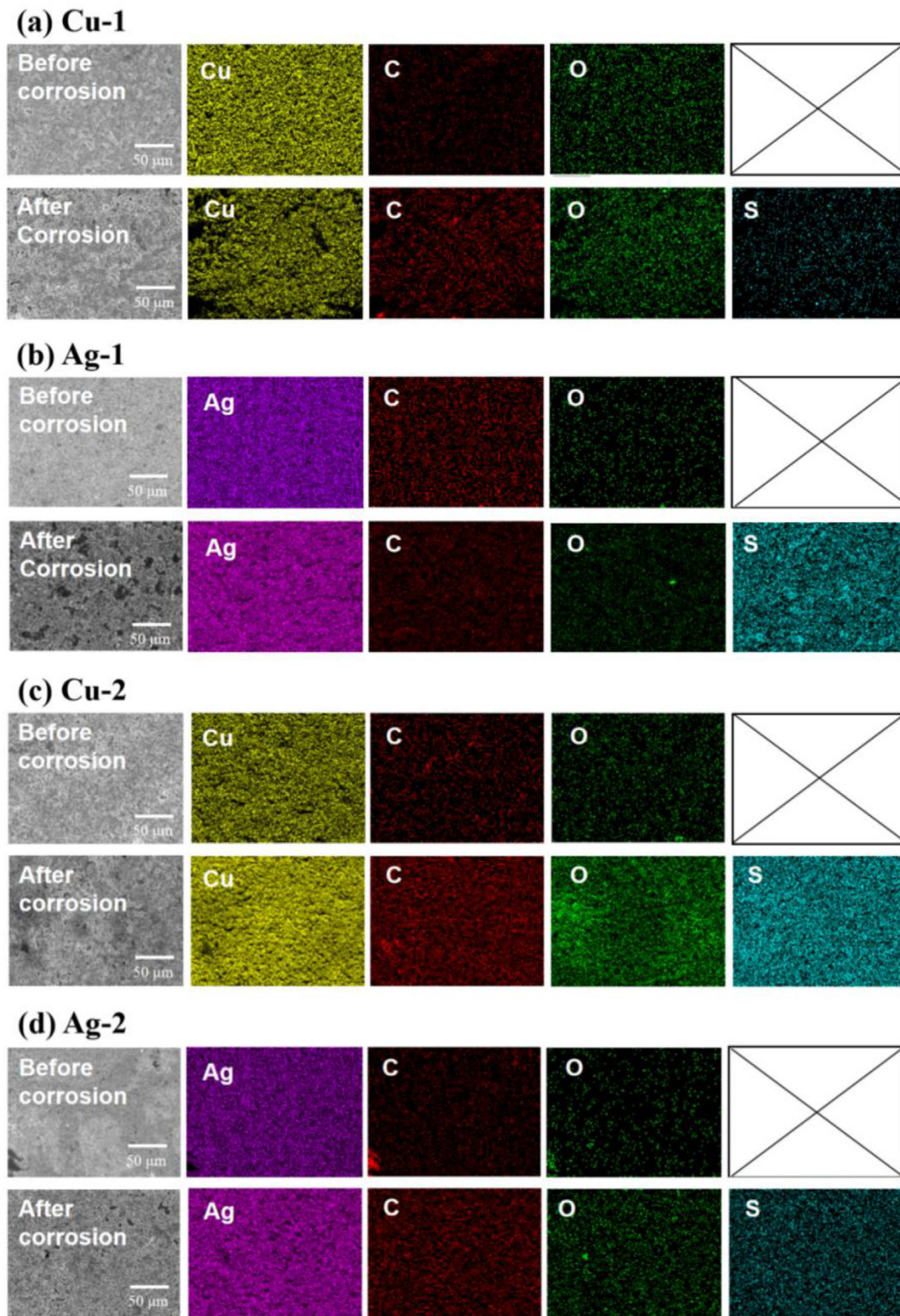
Fig. 11 – EDS elemental mapping images of the surface of cylindrical sintered samples before and after corrosion (a) Cu-1; (b) Ag-1; (c) Cu-2 and (d) Ag-2.
