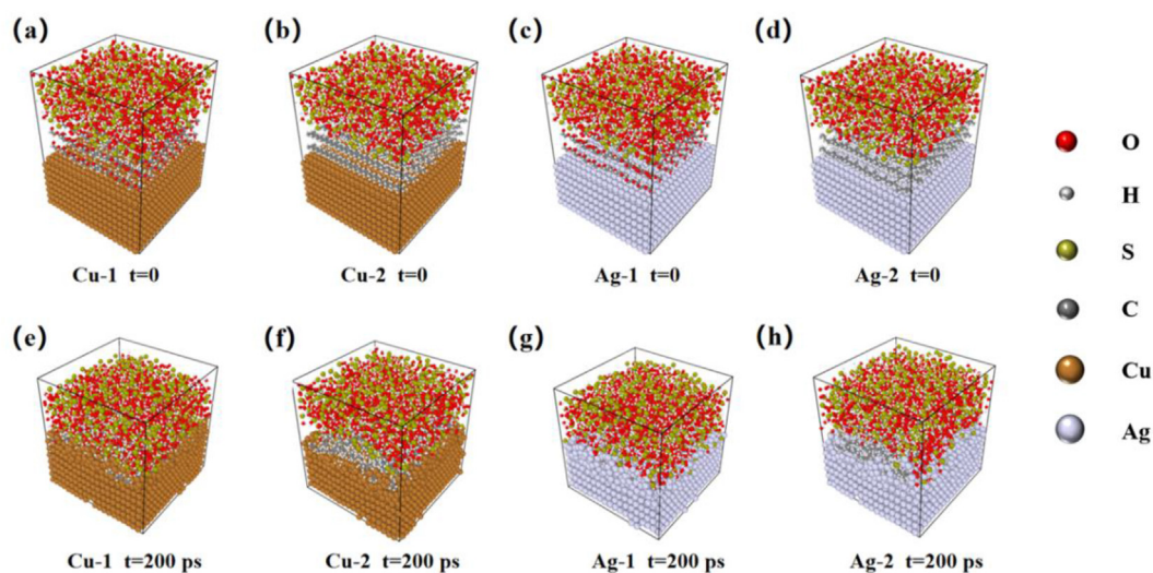
Fig. 16 – (a)–(d) The initial configurations of the simulation model. (e)–(h) Configurations after corrosion simulation (200 ps). (Red is oxygen, white is hydrogen, yellow is sulfur, black is carbon, brown is copper, and gray is silver.).
