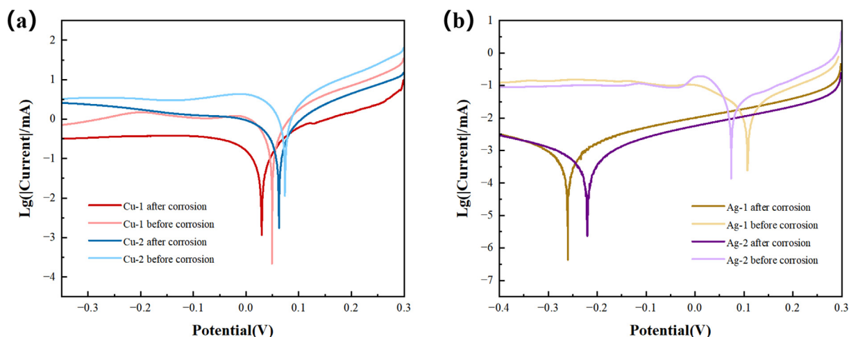
Fig. 14 – The polarization curves of (a) copper-based sintered paste and (b) silver-based sintered paste before and after corrosion.
