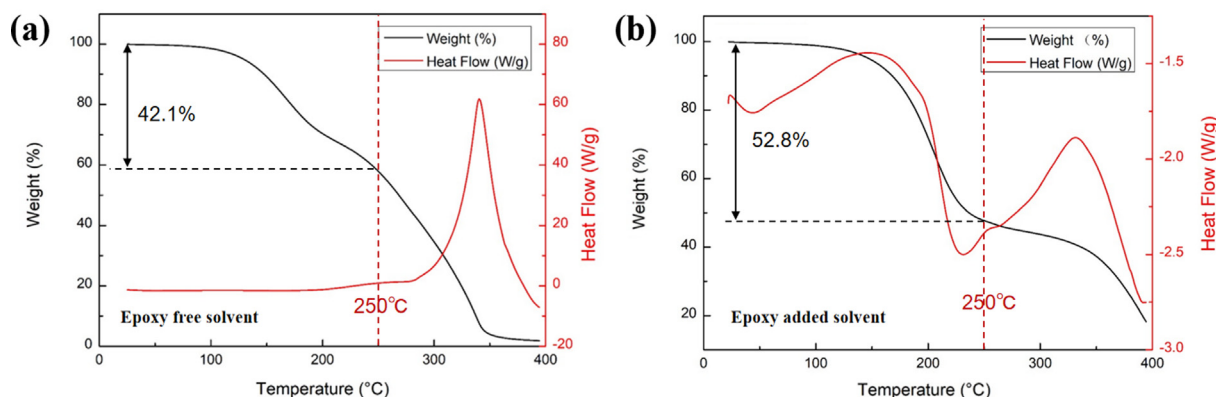
Fig. 3 – Thermal performance analysis of (a) epoxy-free solvent and (b) epoxy-added solvent.
