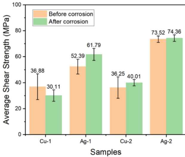
Fig. 7 – Average shear strength of the sintered joints before and after corrosion.
