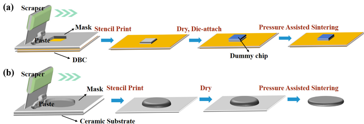
Fig. 4 – Schematic diagram of (a) sintered joint sample preparation and (b) cylindrical sintered sample preparation.
