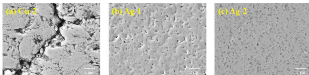
Fig. 21 – SEM photos of the sintered layer in the joints after thermal shock (a)Cu-2; (b)Ag-1; (c)Ag-2.
