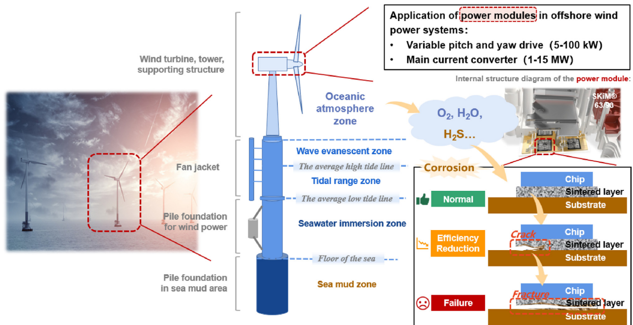
Fig. 1 – The failure diagram of the power module in offshore wind power application.
