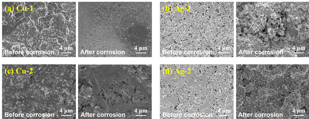
Fig. 10 – Surface SEM photos of the cylindrical sintered samples fabricated by (a)Cu-1; (b)Ag-1; (c)Cu-2 and (d)Ag-2 pastes.
