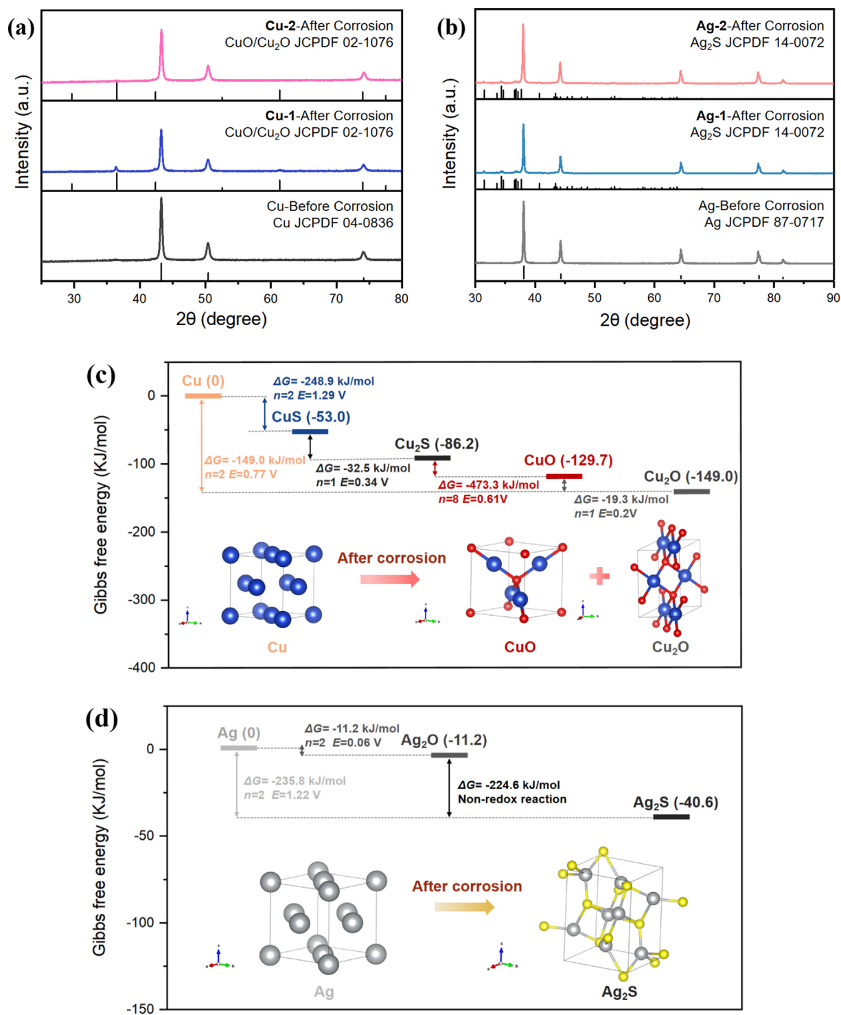
Fig. 12 – XRD test results of the sintered structures before and after corrosion: (a)Cu-1 and Cu-2; (b)Ag-1 and Ag-2. Possible reactions of the sintered (c)copper and (d)silver during corrosion.
