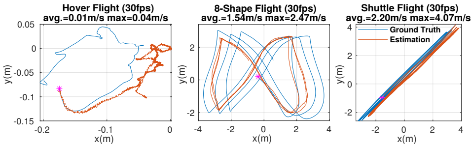
Figure 3.10: The ground-truth and estimated trajectories of hover flight (left), 8-shape flight (middle), and shuttle flight (right).
