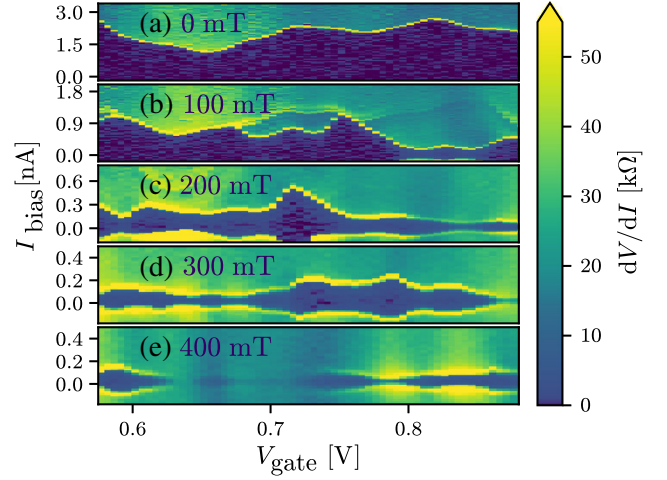
FIG. 3. (a)–(e) dV/dI vs V_g and I_{\text{bias}} at different B (indicated within each panel). Data from device 2. The gate used for tuning is different from that used in Fig. 2, see the Supplemental Material [25]
