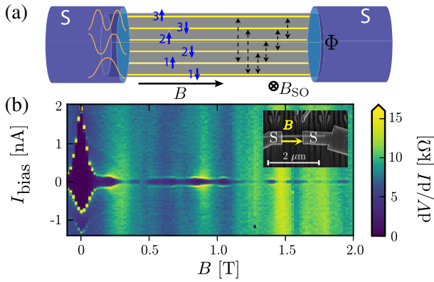
FIG. 1. (a) Schematic superconductor (S)-nanowire-S Josephson junction. The cross section shows cartoon wave functions of n = 3 transverse modes and the flux \Phi penetrating the area of the nanowire. The blue arrows indicate spin-resolved modes; the black dashed arrows are same-spin scattering events within the wire. All modes are coupled at the contacts. The directions of B and the spin-orbit effective field B_{SO} are indicated. (b) Differential resistance dV/dI vs B and I_{bias} . The current bias sweep direction is from negative to positive. Data from device 1. Inset: SEM image of a typical device similar to those studied here. S labels the superconducting contacts while B indicates the in-plane magnetic field for device 2.
