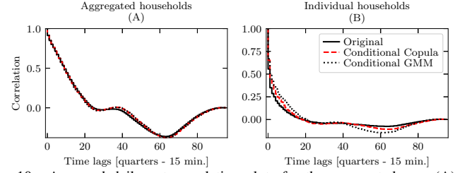
Fig. 10. Averaged daily autocorrelation plots for the aggregated case (A), and the individual case (B) for one year of data.
