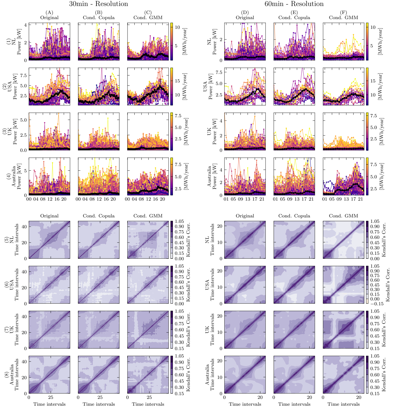
Fig. 13. Simulation results for the smart meter datasets of Table I. Columns (A) and (D) show the original load profiles from one day in June at 30 and 60 minutes resolution. Thick black lines show the median RLP for each dataset. Simulations from the conditional elliptical copula models are shown in columns (B) and (E). Simulations from cond. GMM are in columns (C) and (F). The heat maps of the correlation matrix from (1) to (5) show correlation structures, meaning different consumption profiles patterns from each dataset.
