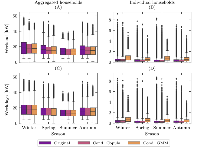
Fig. 8. Load consumption of one year split into seasons, weekends, and weekdays. The conditional multivariate elliptical copula can model the original data set for both aggregated and individual residential consumption cases successfully.
