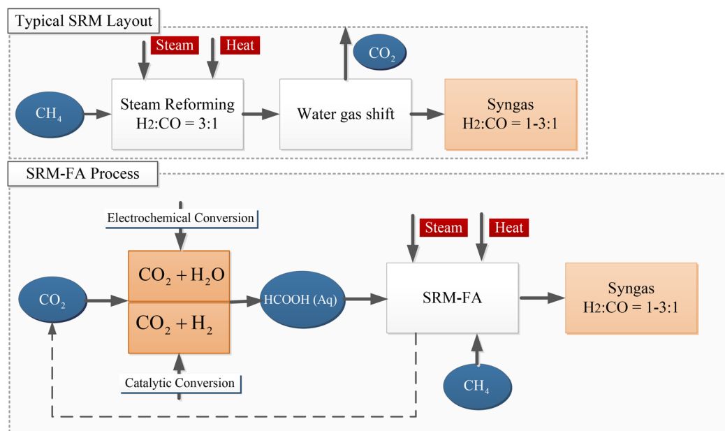
Figure 4. Comparison between a typical SRM layout and the layout for the proposed combined SRM-FA process. In the exiting SRM process, steam reforming is followed by the WGS process to adjust the \text{H}_2:\text{CO} ratio. In the alternative process, first FA is synthesized, and second the FA is added to the SRM to adjust the \text{H}_2:\text{CO} ratio. FA can be synthesized either by electrochemical conversion of \text{CO}_2 9–13 or by conventional catalytic hydrogenation of \text{CO}_2 . 4,18
