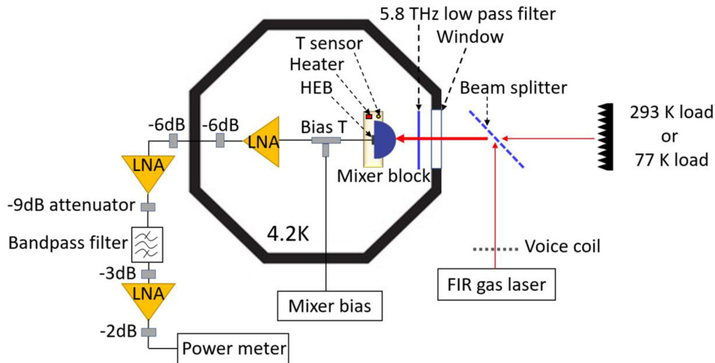
FIG. 2. Schematics of setup-A that is the measurement setup in air for measuring T_{rec}^{DSB} of the HEB-A mixer. It is measured at f_{if} = 2 GHz with a narrow band ( \Delta f_{if} ) of 100 MHz, defined by the bandpass filter.
