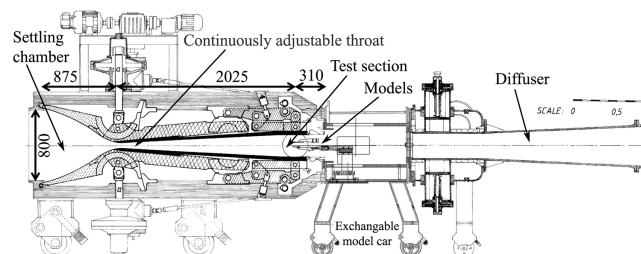
Fig. 3 TST-27 in supersonic configuration (adapted with permission from Giepman [10]).
