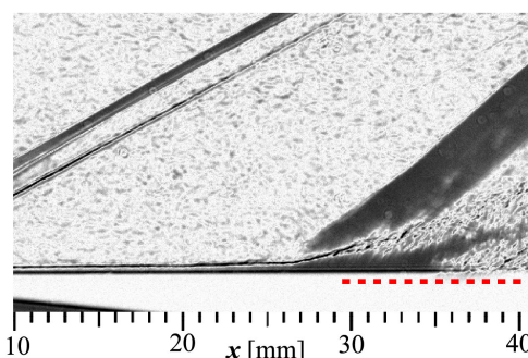
c) Collapsed laminar part of separation bubble. No visible laminar separation shock. Turbulence (red) at x = 30 mm
