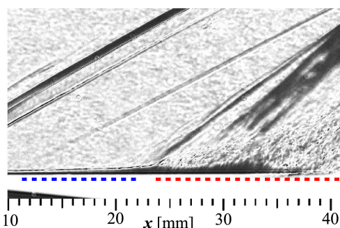
b) Collapse of laminar part (blue). Laminar separation shock at x = 11 mm vanishing. Turbulence (red) at x = 24 mm
