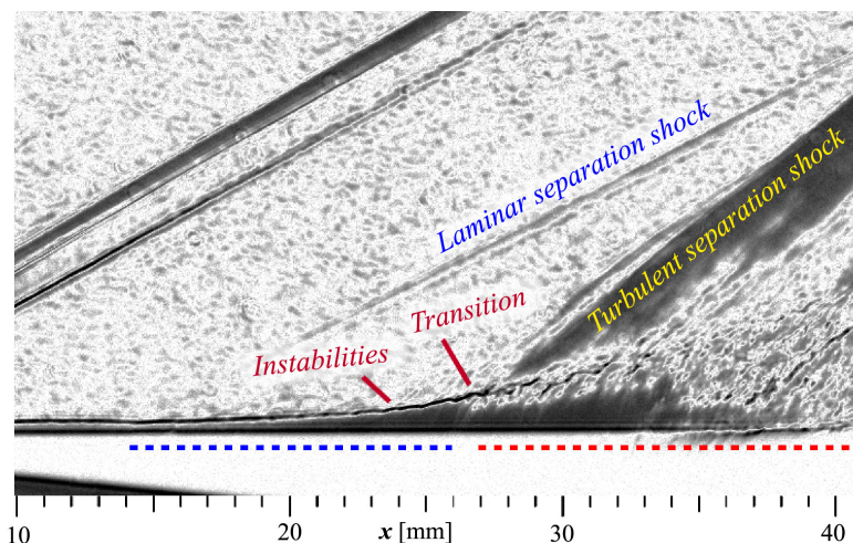
a) Growth phase of laminar part (blue). Laminar separation shock at x = 14 mm, transition at x = 27 mm
