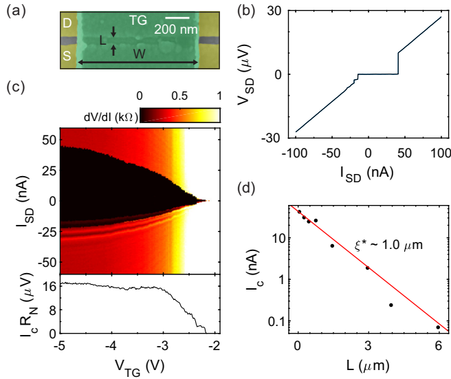
FIG. 1. (a) False-color SEM image of a planar Josephson junction device with width W = 1 \mu\text{m} and length L = 50 \text{ nm} . The top gate (TG, indicated in green) is used to induce a 2DHG in the strained germanium quantum well contacted by a superconducting Al source (S) and drain (D) lead, depicted in yellow. (b) IV curve of a junction with L = 50 \text{ nm} at V_{\text{TG}} = -4 \text{ V} , showing a clear supercurrent with I_S = 43 \text{ nA} . (c) Color plot of the differential resistance of the junction dV/dI as a function of the bias current I_{\text{SD}} and top-gate voltage V_{\text{TG}} (top panel) and derived I_S R_N product as a function of V_{\text{TG}} (bottom panel). (d) Length dependence of the supercurrent. A purely exponential decay is observed over the entire junction length range, with a decay length of 1.0 \mu\text{m} .
