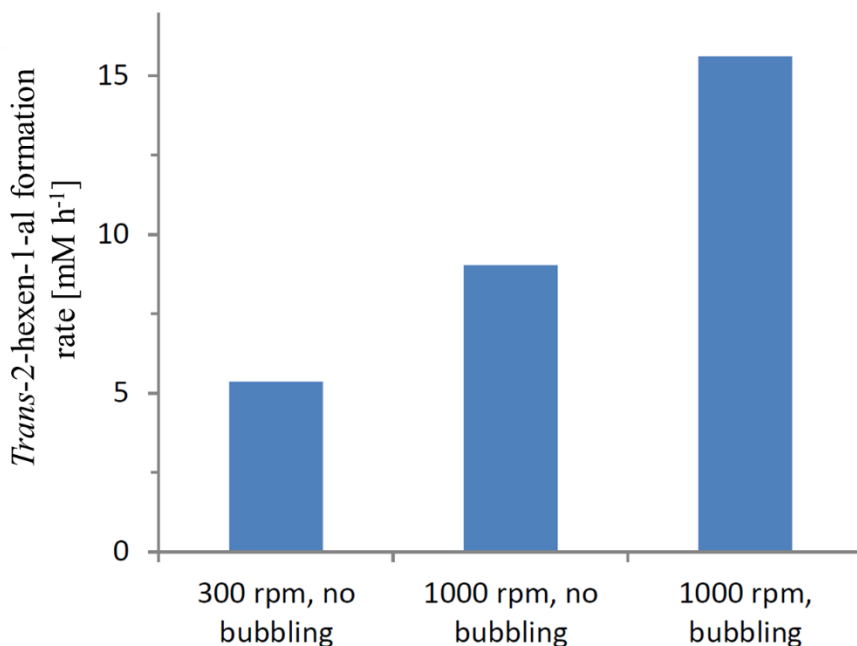
Figure 5 Influence of \text{O}_2 -supply on the rate of the PeAAOx -catalysed oxidation of trans -2-hexen-1-ol. Conditions: potassium phosphate buffer (1 mL, 50 mM, pH 7.0) containing 0.05\text{ }\mu\text{M} PeAAOx , 720\text{ U mL}^{-1} catalase and 50 mM trans -2-hexen-1-ol.
