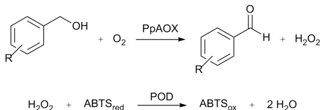
Scheme 2 Spectrophotometric assay to determine the activity of PpAOX . PpAOX : alcohol oxidase from Pichia pastoris , ABTS TM : 2,2'-azino-bis-(3-ethylbenzothiazoline-6-sulfonic acid), POD : peroxidase from horseradish.
