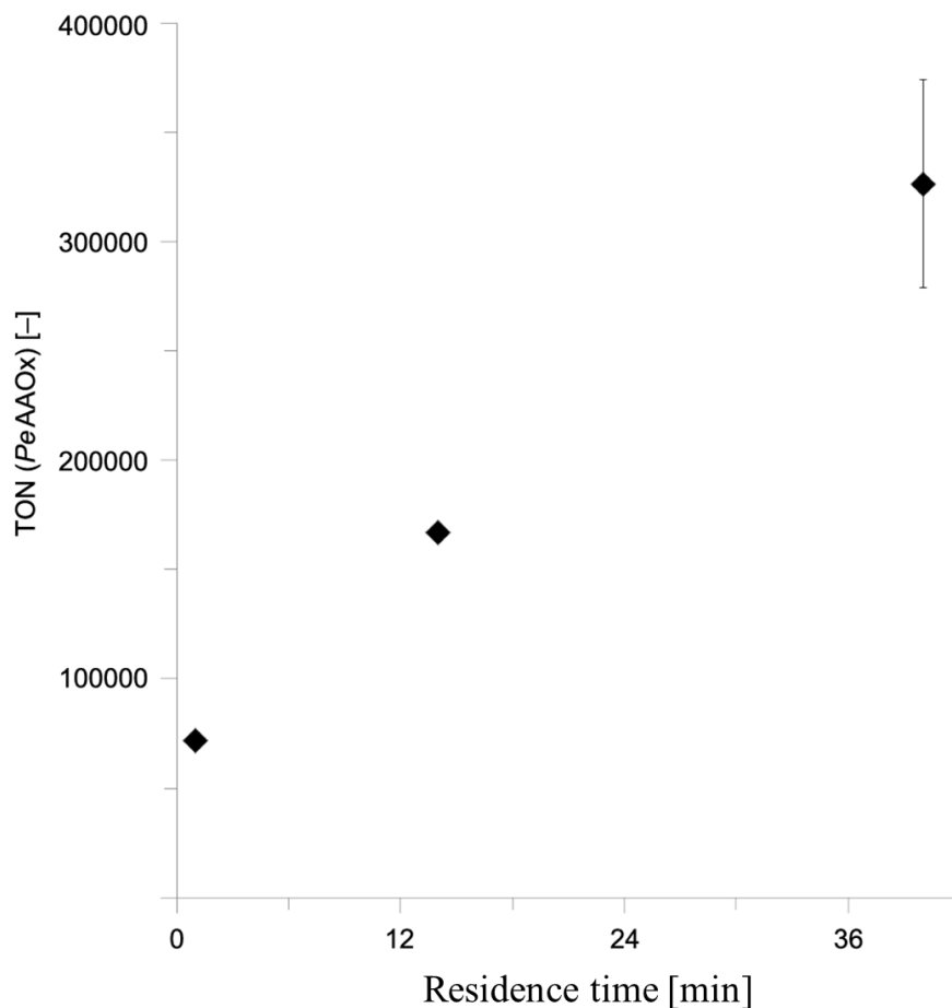
Figure 6 Increasing the PeAAOx turnover numbers (TN) by increasing the residence time. Conditions: 6 mL flow reactor, 50 mM KPi buffer (pH 7, 30 °C), [trans\text{-}2\text{-hexen-1-ol}]_0 = 40\text{ mM} , [PeAAOx] = 0.02\text{ }\mu\text{M} , [catalase] = 600\text{ U mL}^{-1} . The TN value was calculated based on the GC yield of every run. The TN was obtained by dividing the product concentration (determined chromatographically) by the biocatalyst concentration.
