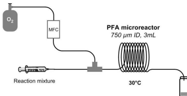
Scheme 2 - View of the reaction setup. The oxygen gas flow was controlled by a mass flow controller (MFC), and a syringe pump controlled the reaction mixture flow. The sample was collected on ice or directly in ethyl acetate at the end of the reactor.
