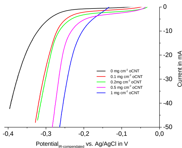
Figure 1 Linear sweep experiments of electrodes modified with different amounts of oCNTs in 100 \text{ mM} sodium citrate ( \text{pH } 5 ) with 100 \text{ mM} KBr. Potentials are iR-compensated.
