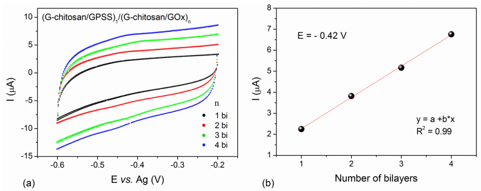
Figure 5 (a) Cyclic voltammograms conducted at 80 mV.s -1 scan rate for 1, 2, 3 and 4 bilayers and (b) plot of the anodic peak vs. the number of bilayers for (G-chitosan/ GPSS) 1 /(G-chitosan/GOx) 4 immersed in aqueous 0.1M PBS pH 6.2.
