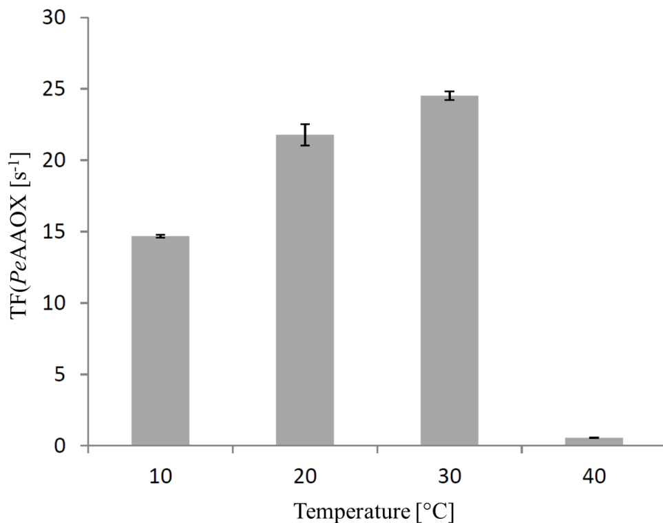
Figure 2 Influence of temperature on the activity of PeAAOx . Reactions performed at 10, 20, 30 or 40°C and 1000 rpm in potassium phosphate buffer (1 mL, 50 mM, pH 7.0) containing 0.05 \mu M PeAAOx , 720 U mL -1 catalase and 50 mM trans -2-hexen-1-ol.
