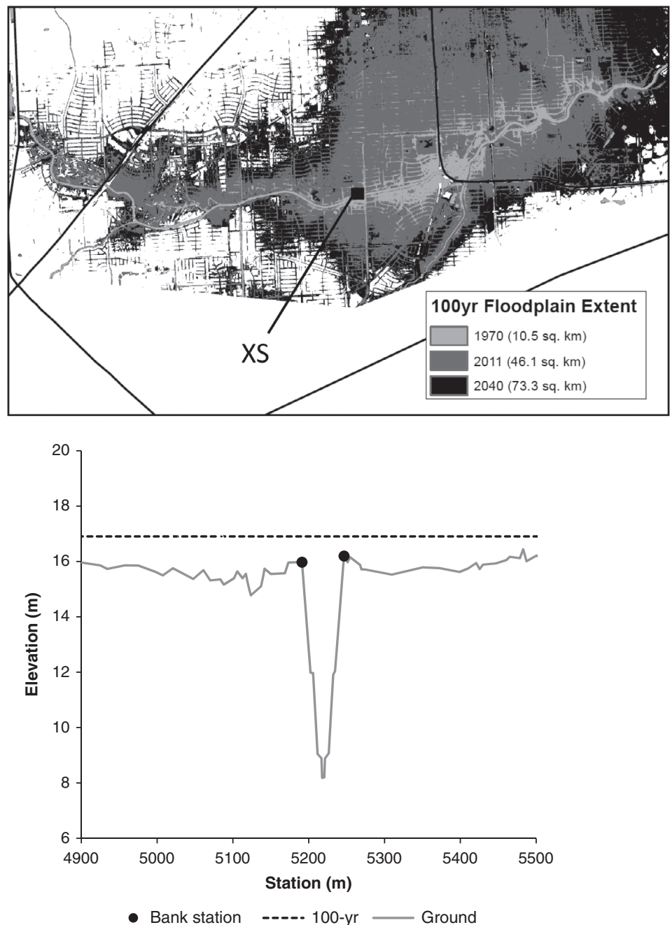
FIGURE 9 100-year floodplain with selected cross-sectional (XS) view at Brays Bayou
