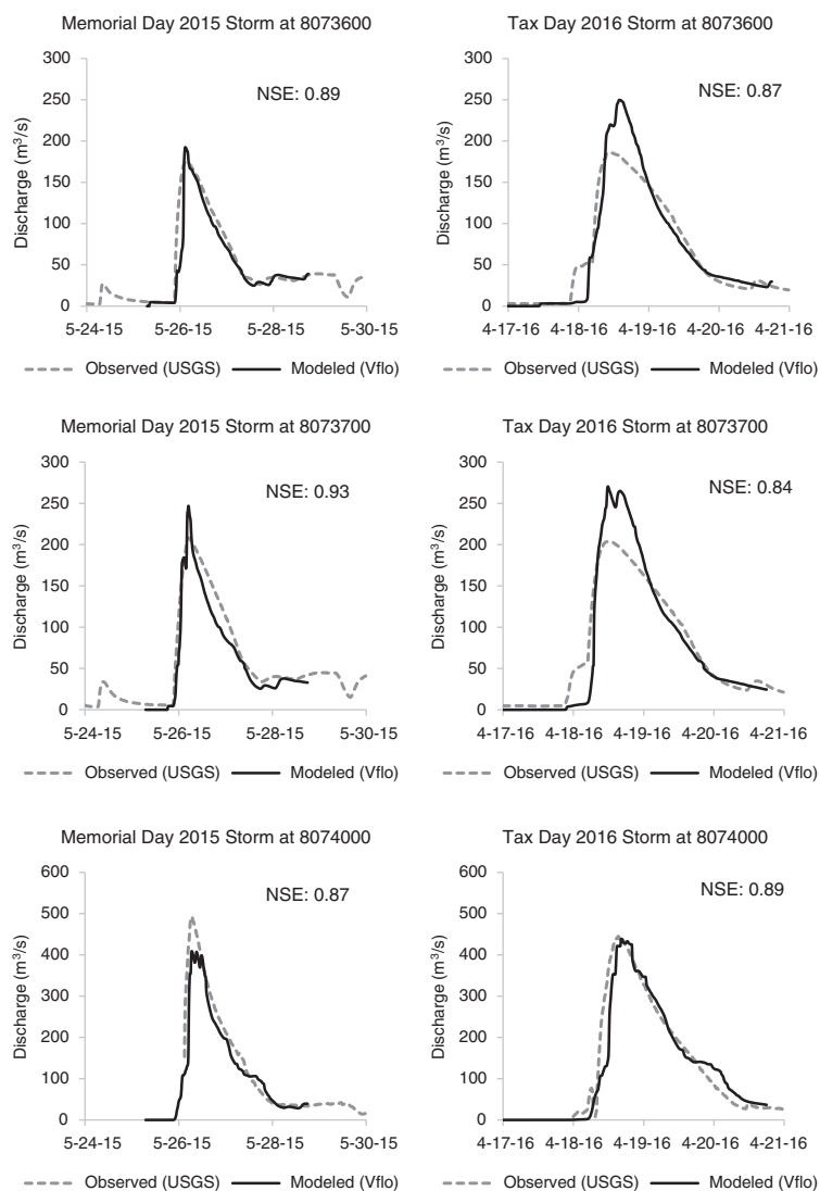
FIGURE B1 Stream flow comparisons in Buffalo Bayou
