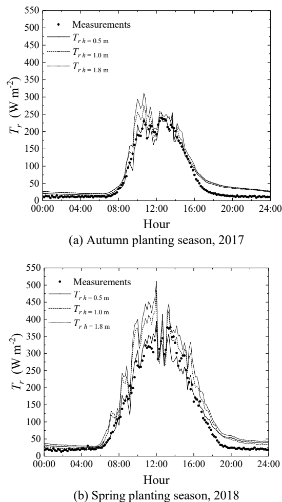
Figure 7. Variations of the measured and estimated average T_r values by the Stanghellini model (SM) based on the meteorological data at three observation heights (a) from 2 to 10 November 2017 and (b) from 2 to 10 May 2018.
