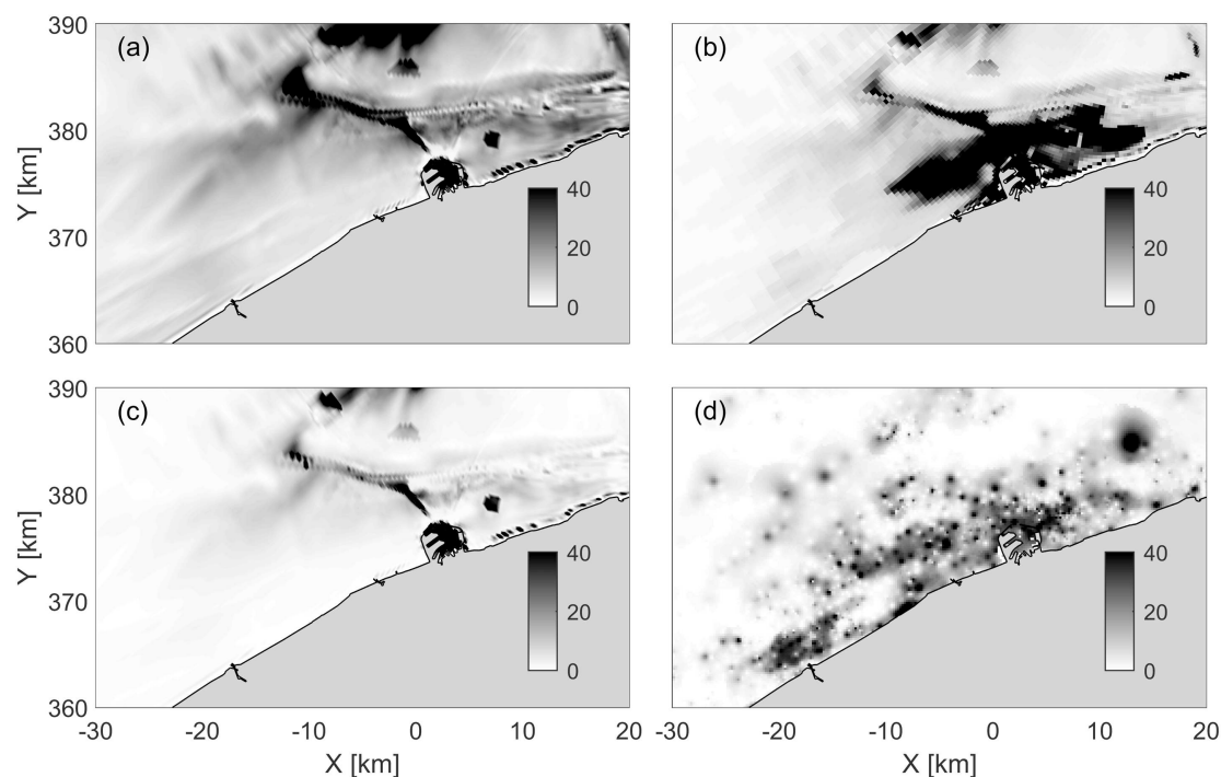
Fig. 10. Amount of mud in the bed computed by the model for the reference model (a), model alternative 1 (mud source, b) and model alternative 2 (reduced deposition, c), in \text{kg/m}^2 (sum of layer 1 and 2, and all mud fractions). Panel d provides the measured clay fraction (from Fettweis et al., 2009b ) in %.
