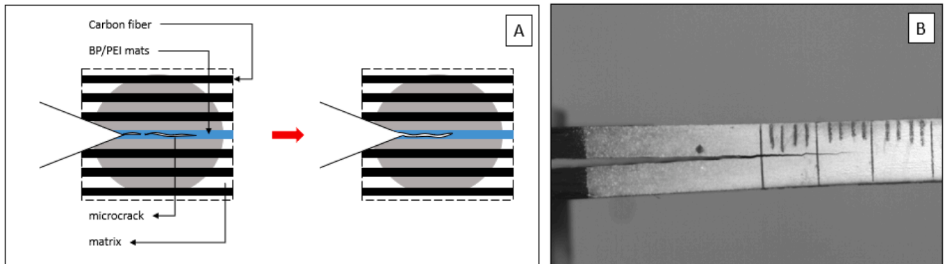
Fig. 10. (A) Scheme of the crack formation and its propagations for PEEK/BP/CF and PEI/BP/CF, and (B) real example of initial straight crack propagation observed during the test.
