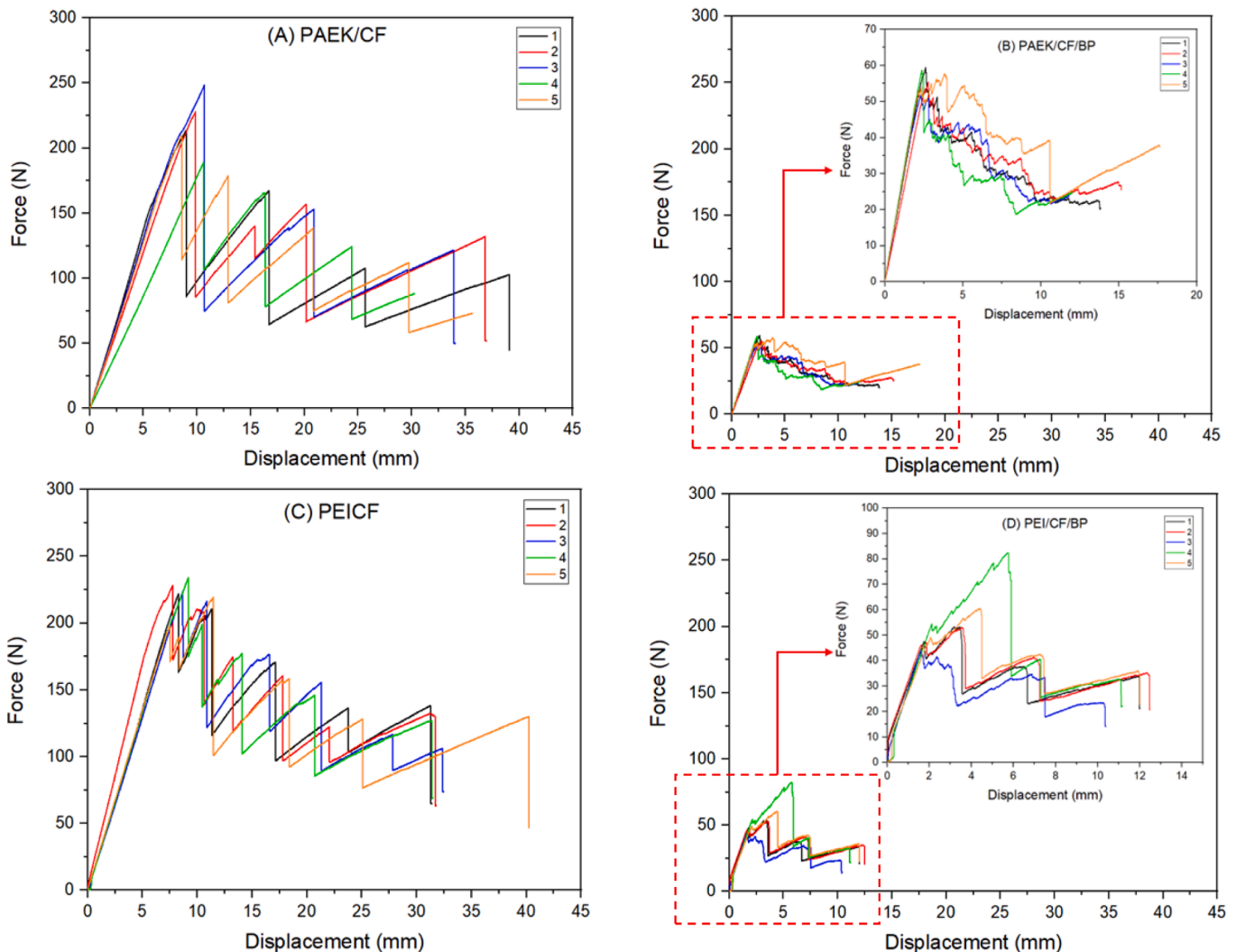
Fig. 4. Load-displacement curves obtained via DCB (mode-I) test for (A) PAK/CF, (B) PAK/BP/CF, (C) PEI/CF, and (D) PEI/BP/CF laminates.
