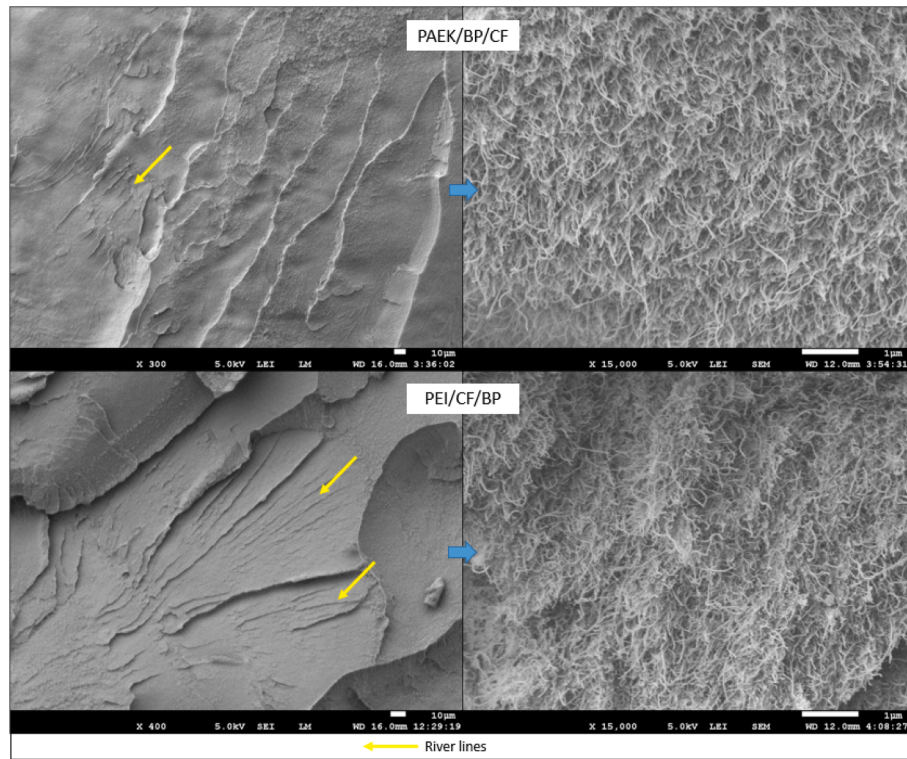
Fig. 8. SEM micrographs of the mode-I fracture surface for PAEK and PEI/BP/CF with river lines (yellow arrows) along the surface. (For interpretation of the references to colour in this figure legend, the reader is referred to the web version of this article.)
