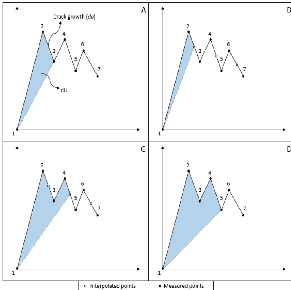
Fig. 3. Scheme of how quasi-static data was used to obtain dU/dN and da/dN from mode-I and mode-II tests (a) observed crack growth, (b) half, (c) one and half, and (d) two of the observed crack growth ( da ).
