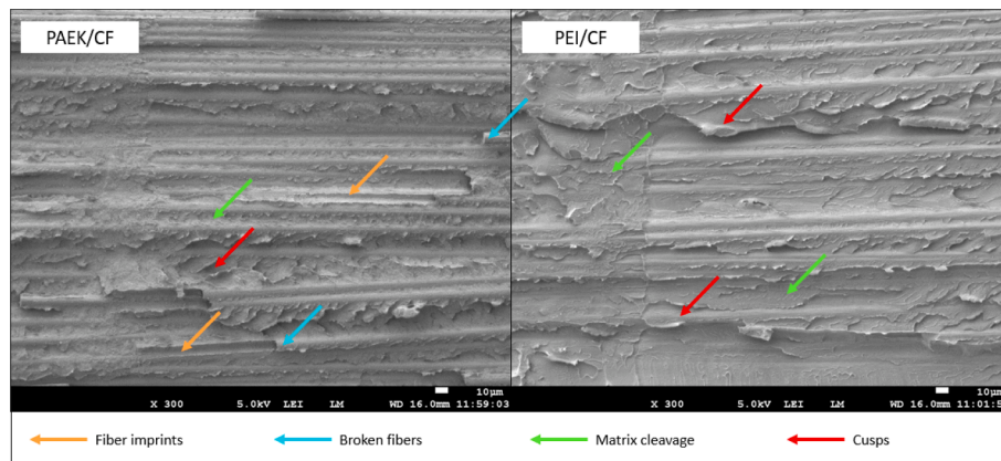
Fig. 7. SEM micrographs of the mode-I fracture surface for PAEK/CF and PEI/CF. The mechanisms observed are broken fibers (blue arrows), matrix cleavage (green arrows), cusps (red arrows), and fiber imprints (orange arrows). (For interpretation of the references to colour in this figure legend, the reader is referred to the web version of this article.)
