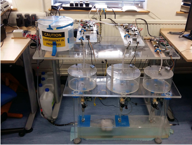
Figure 6.6: WaterBox testbed.
