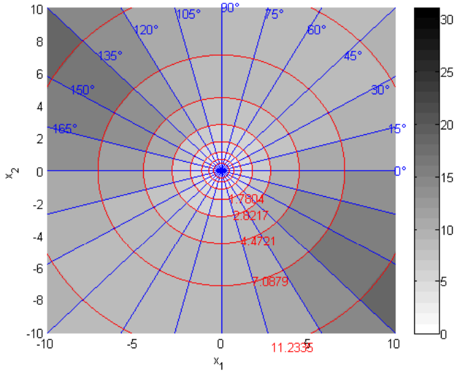
Figure 5.4: Zoomed-in result of the regional lower bound with W = 2 .
