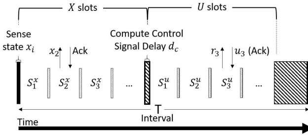
Figure 6.3: C-TDMA protocol.
