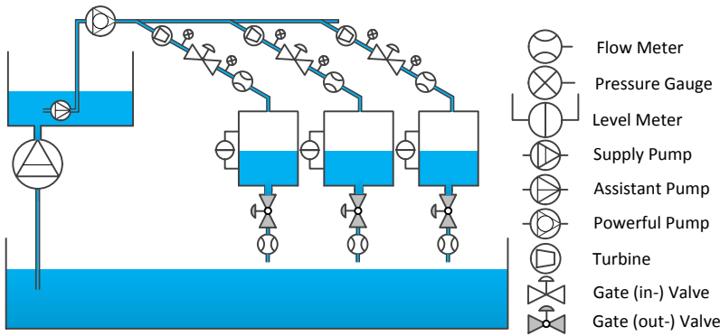
Figure 6.7: WaterBox schematic structure.
