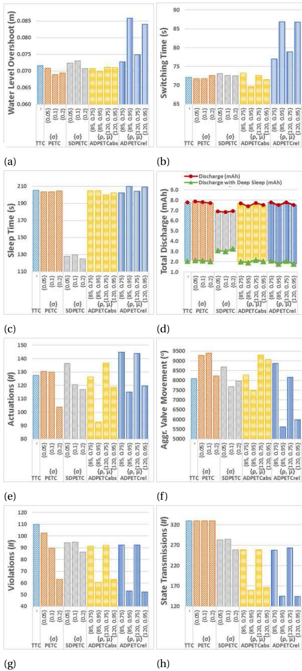
Figure 6.12: Impact of ETC parameters ( \sigma , \mu , \rho ) in: (a) water level overshoot, (b) switching time, (c) sleep time, (d) discharge, (e) actuations, (f) valve movement, (g) violation, and (h) state transmissions.
