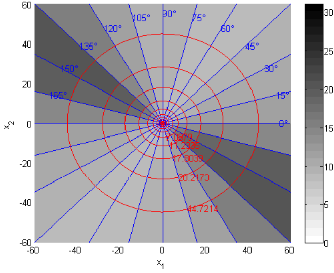
Figure 5.3: Computed result of the regional lower bound with W = 2 .
