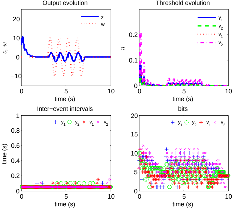
Figure 3.3: Simulation result when w(t) = 10 \sin(2\pi t) , t = [3, 7] : evolution of z and w , threshold, inter-event intervals, and bits of each event.
