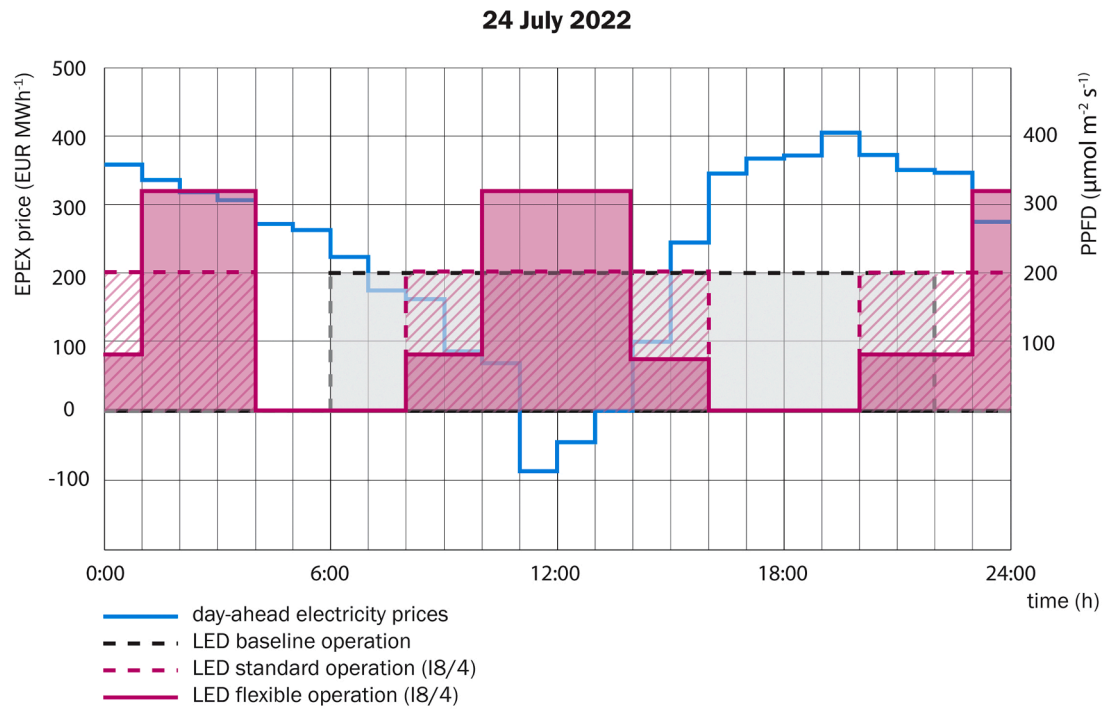
Fig. 12b. LED operation I8/4 standard versus flexible operation on July 24th, 2022.
