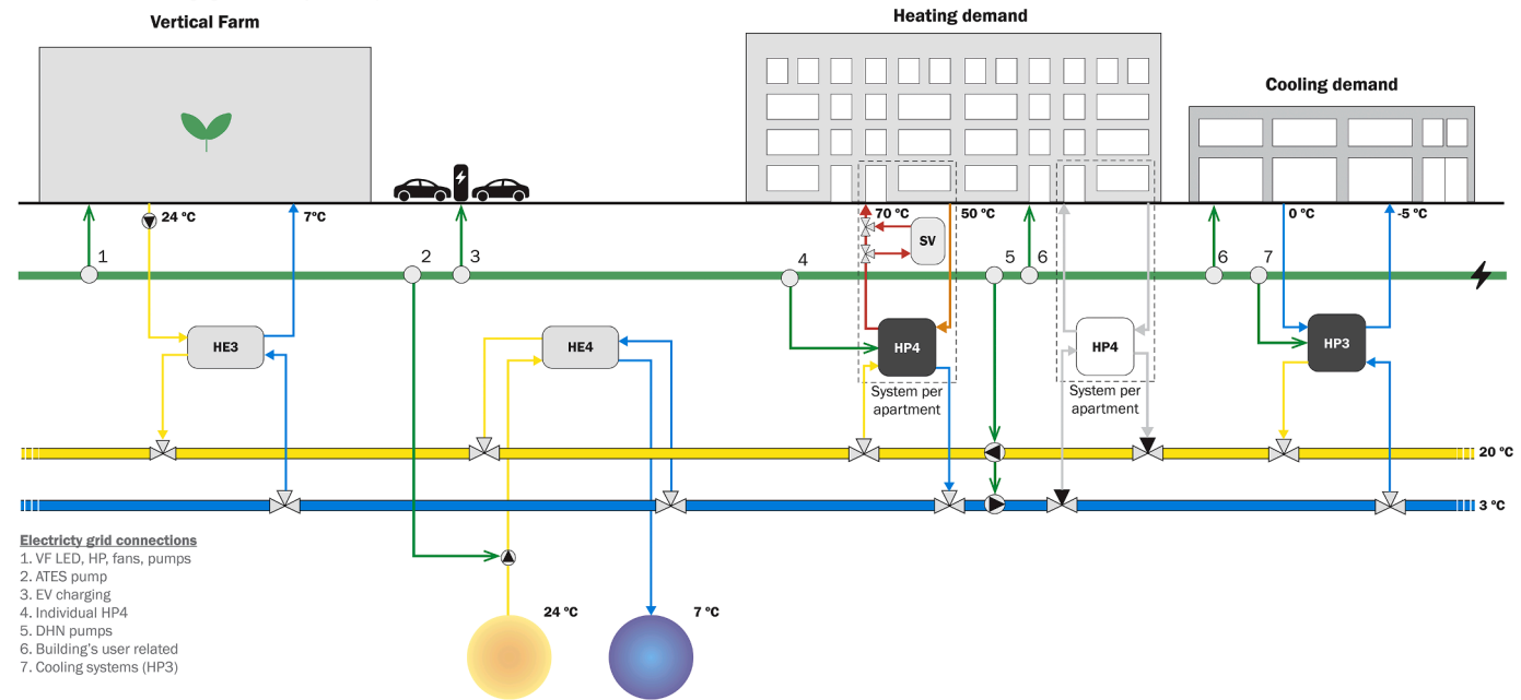
Fig. 8. Decentralised energy system configuration with 2-pipe DHN in winter mode.
