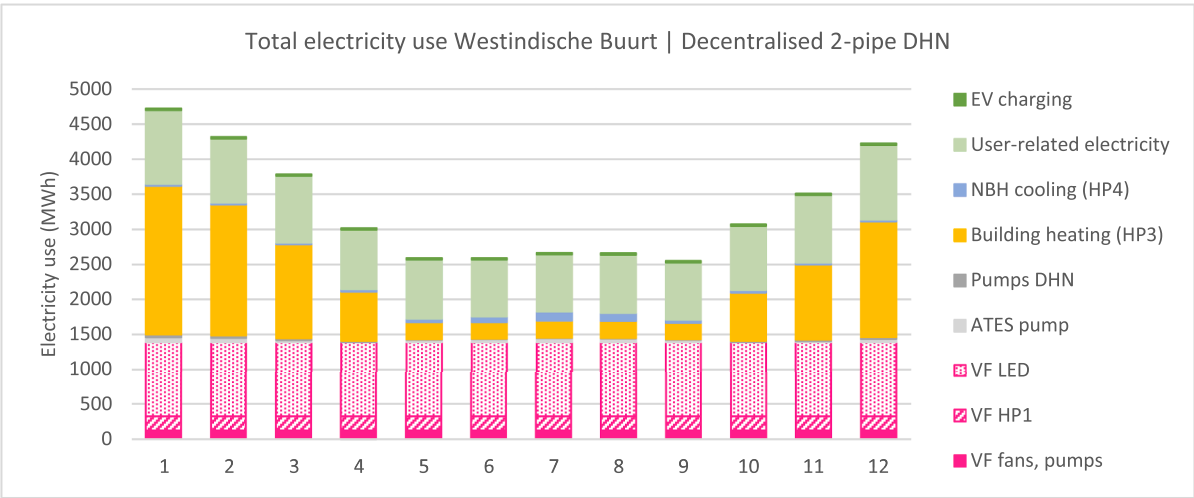
Fig. 9. Annual electricity use of the Westindische Buurt with integrated VF using the decentralised 2-pipes DHN configuration.
