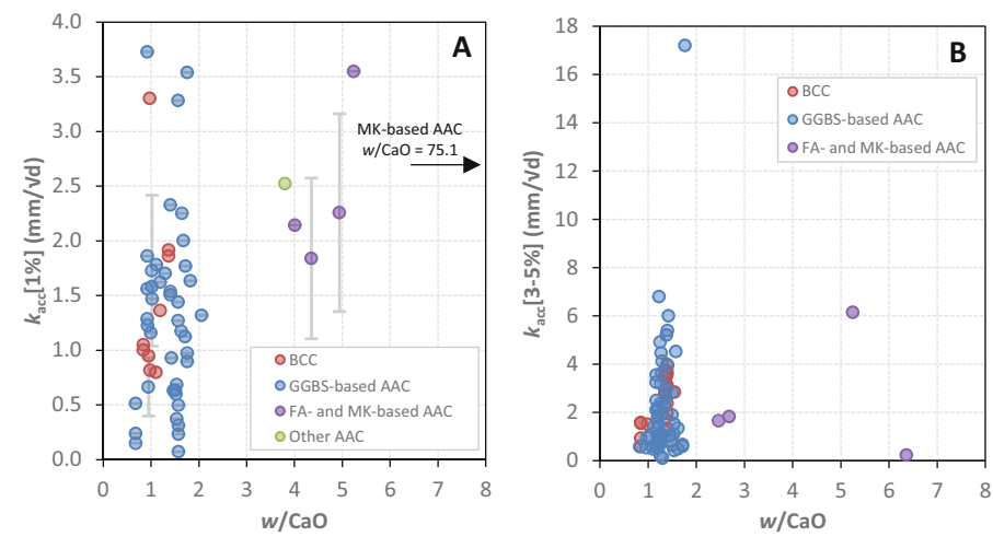
Fig. 6. Carbonation coefficients obtained under accelerated conditions (A, c_{CO_2} = 1\% ; B, c_{CO_2} = 3\text{--}5\% ) versus w/\text{CaO} ratio. Error bars represent the estimated standard deviations of the results obtained by RILEM TC 247-DTA.
