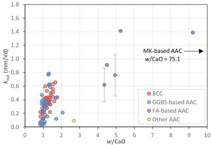
Fig. 1. Carbonation coefficients obtained under conditions approximating natural carbonation versus w/CaO ratio. Error bars represent the estimated standard deviations of the results obtained by RILEM TC 247-DTA.
