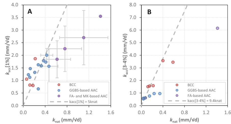
Fig. 5. Carbonation coefficients obtained under accelerated conditions (A, c_{CO_2} = 1\% ; B, c_{CO_2} = 3\text{--}4\% ) versus the carbonation coefficients obtained under conditions approximating natural exposure. Error bars represent the estimated standard deviations of the results obtained by RILEM TC 247-DTA.
