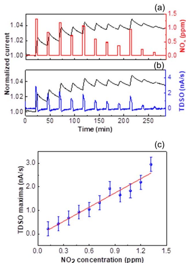
Figure 7. (a) Real-time current behavior of Device 2B towards Test 4 (red rectangles). (b) Differential current (blue curve) overlapped to the current signal (black curve) reported in panel (a). In both panels, the current is normalized to the value of the initial unperturbed state of the first exposure. (c) Values of the maxima of the differential current from plot (b) reported as function of \text{NO}_2 concentrations with the fitting curve (red line).
