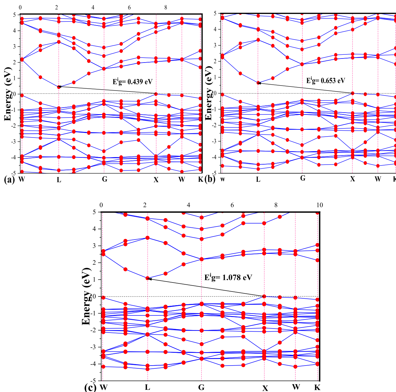
FIGURE 2 (A–C) Band structures of K_2AgBiI_6 by using LDA, GGA, and mGGA, respectively.
