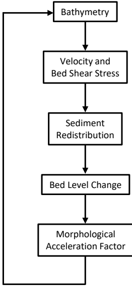
Figure 4.4: Schematic of classical morphodynamic loop (for sandy settings; adapted from Ranasinghe et al. [13]) and refined schematic for erosion-limited fine sediment settings.
