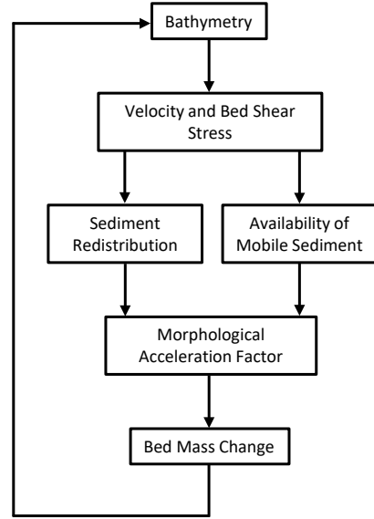
Figure 4.4: Schematic of classical morphodynamic loop (for sandy settings; adapted from Ranasinghe et al. [13]) and refined schematic for erosion-limited fine sediment settings.
