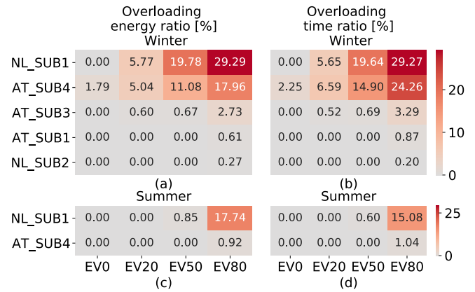
(ii) Heat map of grid congestion duration index: overloaded energy and time ratio
