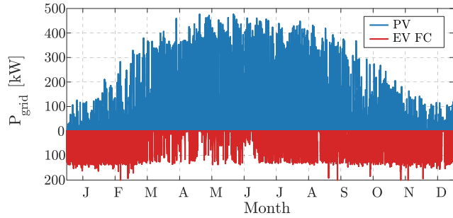
FIGURE 2. PV-FCS power exchange with the distribution grid. The power flow above zero represents the power produced by the solar plant, while the one below zero the power demand due to EV charging.
