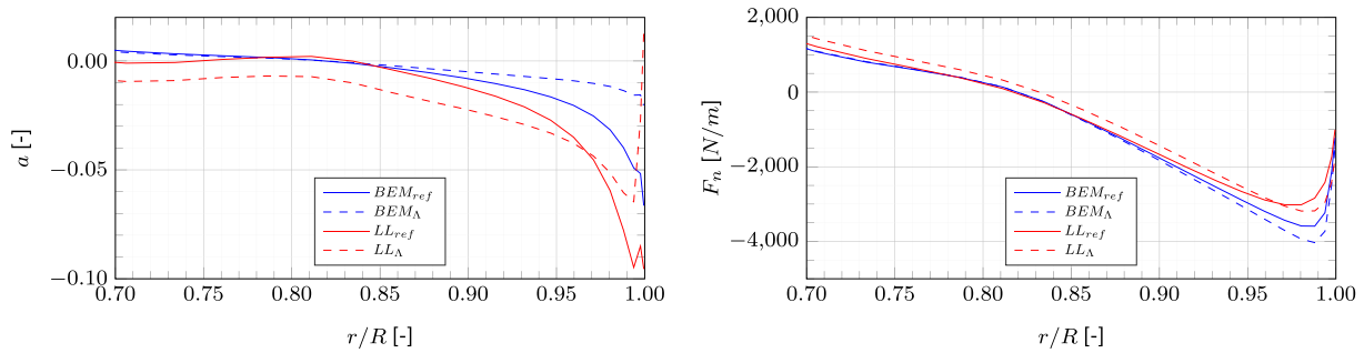
FIGURE 15 Spanwise distribution of axial induction (left) and normal force (right), case: U = 25 m/s, \lambda = 3.8 , \beta_{pitch} = 22.91^\circ , y_{start} = 0.5R , x_{tip} = -0.2R , \gamma = 2
