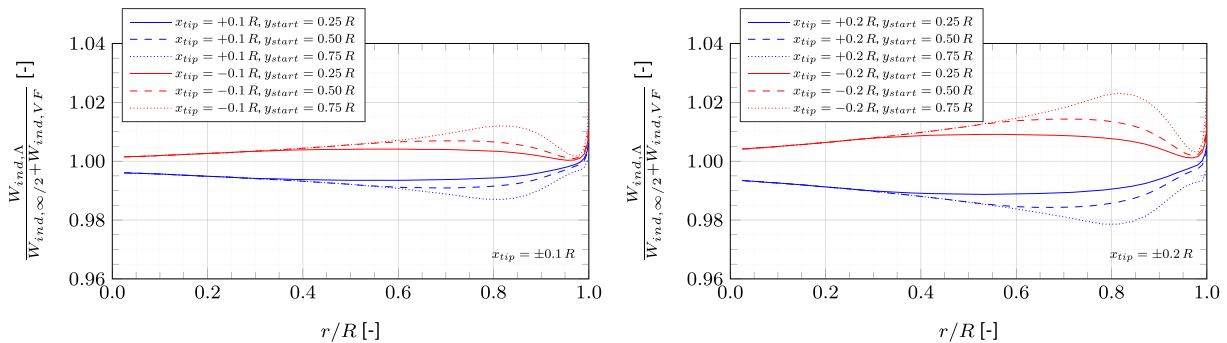
FIGURE 6 Ratio of induced axial velocity simulated using a lifting line approach to the sweep model for swept geometries with x_{tip} = \pm 0.1R (left) and x_{tip} = \pm 0.2R (right)
