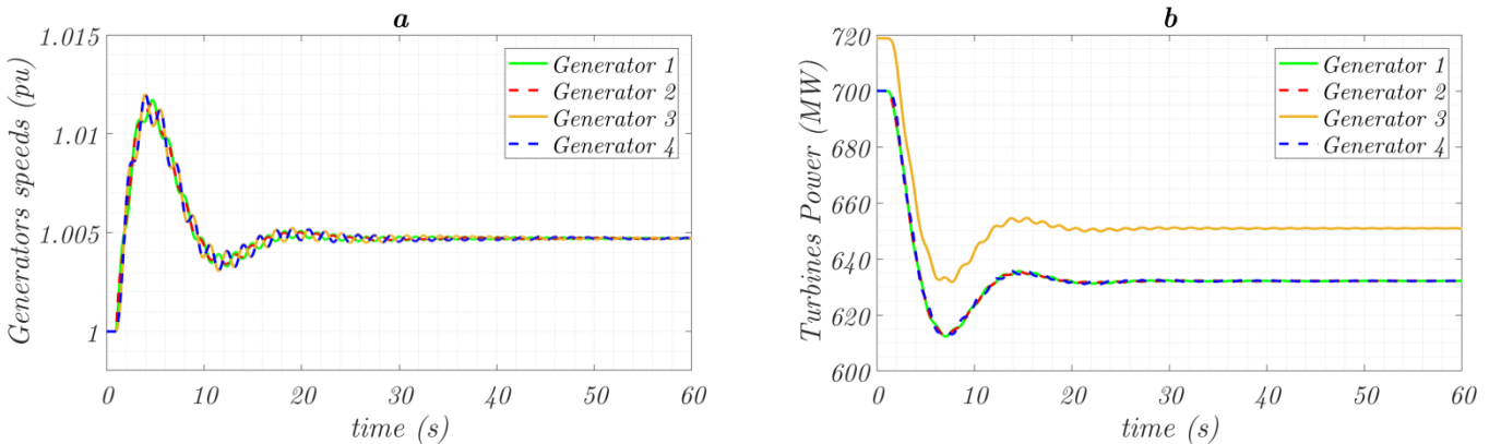
Figure 4. Generators speeds and turbines power responses of the original benchmark system [1] under the Load A1 (cf. Figure 1) disconnection event.
