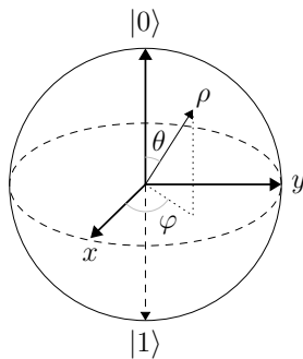
Figure 2.1: Three dimensional representation of a qubit \rho in the Bloch sphere.
