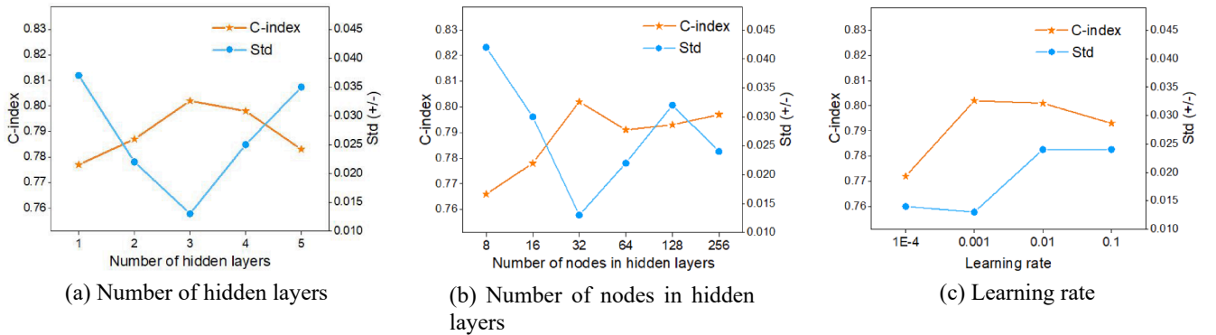
Fig. 4. C-index and Std of different (a) Number of hidden layers, (b) Number of nodes in hidden layers, and (c) Learning rate.
