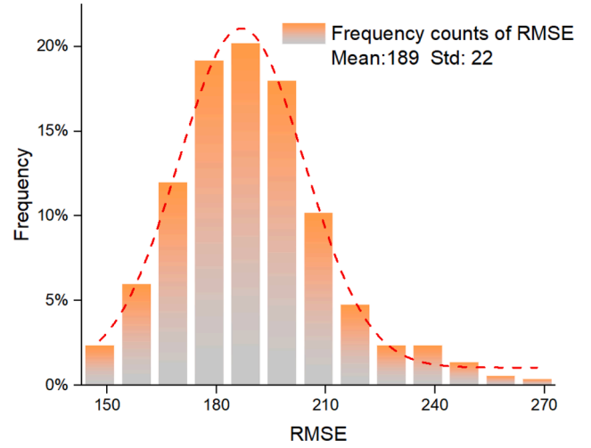
Fig. 8. The distribution of RMSE results for 500 times with the MC dropout on.
