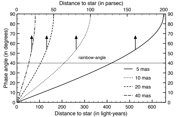
Fig. 14. Observable phase angles for a planet at 1 AU of its star as a function of the observer's distance to the star. Different lines show results for different inner working angles (IWA). The solid line at \alpha = 40^\circ corresponds to the angle at which the rainbow appears, assuming water droplets. For the phase angle range 90^\circ – 180^\circ , the graph mirrors this one over \alpha = 90^\circ .
