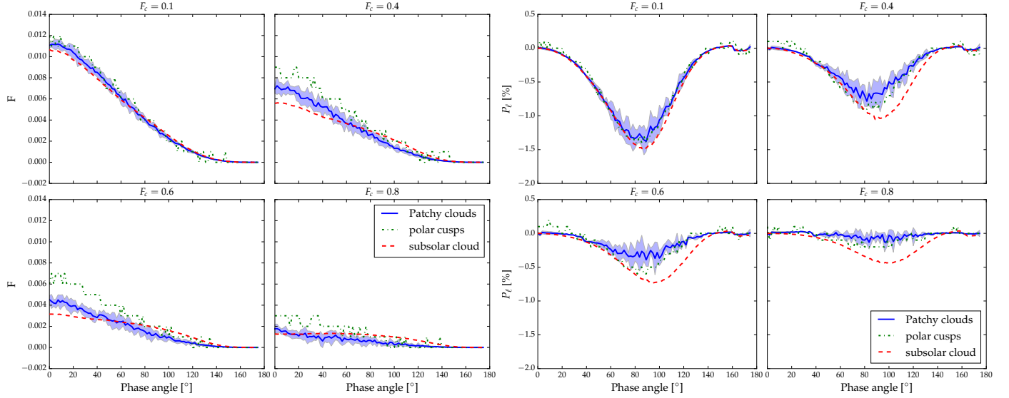
Fig. 10. Differences F^{\text{glint}} - F^{\text{black}} (left) and P_\ell^{\text{glint}} - P_\ell^{\text{black}} (right) at \lambda = 300 nm, as functions of the phase angle \alpha for different cloud coverage types and values of F_c .
