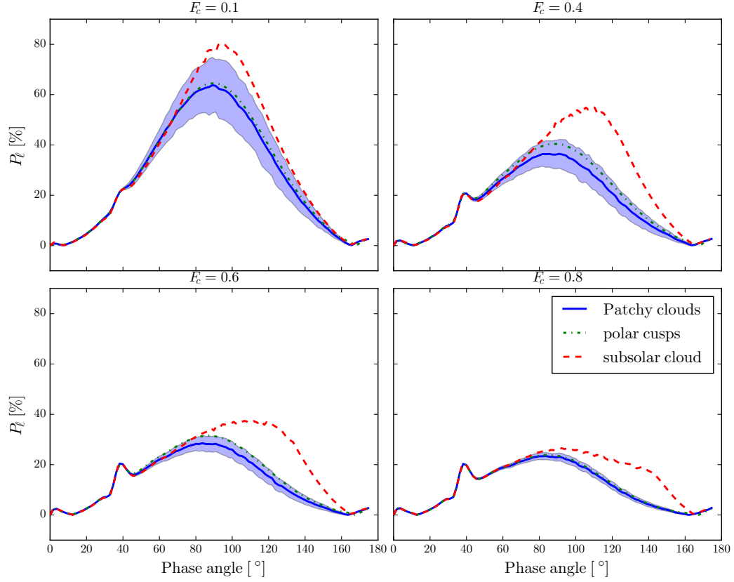
Fig. 6. Comparison of P_\ell at \lambda = 500 nm for different types of cloud cover for F_c = 0.1, 0.4, 0.6 , and 0.8 . The cloud-top pressure p_c is 800 mb. The solid line shows the average of 300 patchy cloud patterns. The shaded area shows the variability of the 300 curves.
