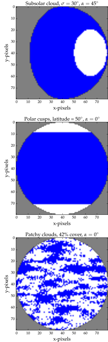
Fig. 1. Examples of our three types of cloud cover on a 80 \times 80 pixel grid: a) sub-solar clouds for \sigma_c = 30^\circ and \alpha = 45^\circ ; b) polar cusps for L_t = 50^\circ and \alpha = 0^\circ ; c) patchy clouds for F_c = 0.42 and \alpha = 0^\circ .
