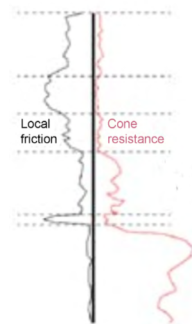
Cone Penetration Test (CPT) data
