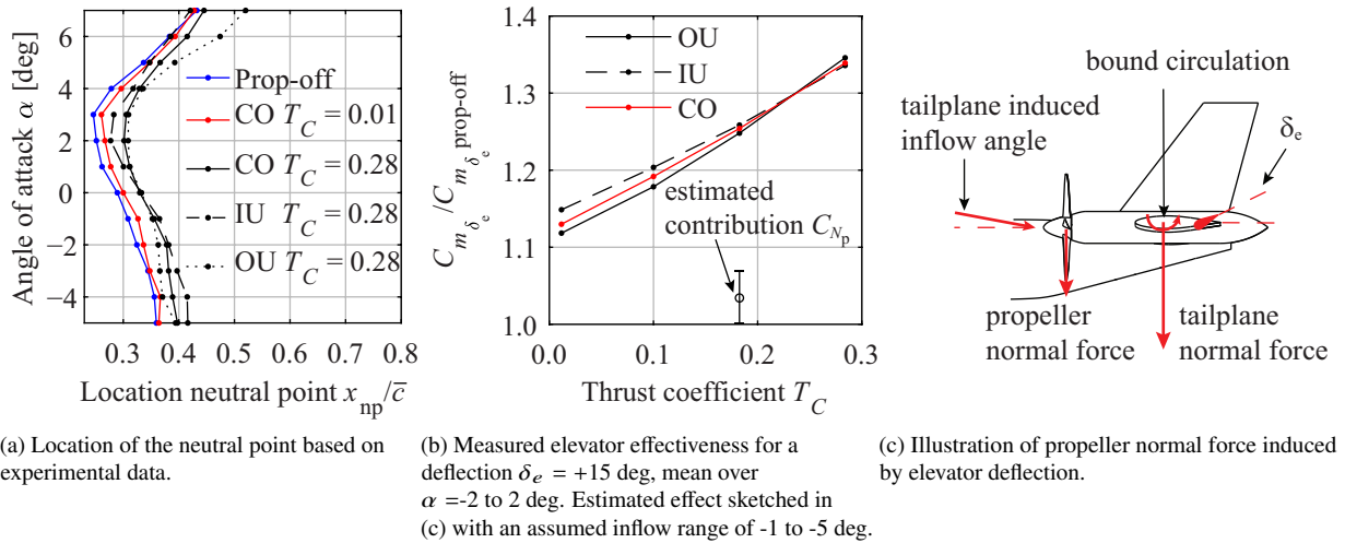
Fig. 14 Effect of propeller installation on location of neutral point and on the elevator effectiveness.
