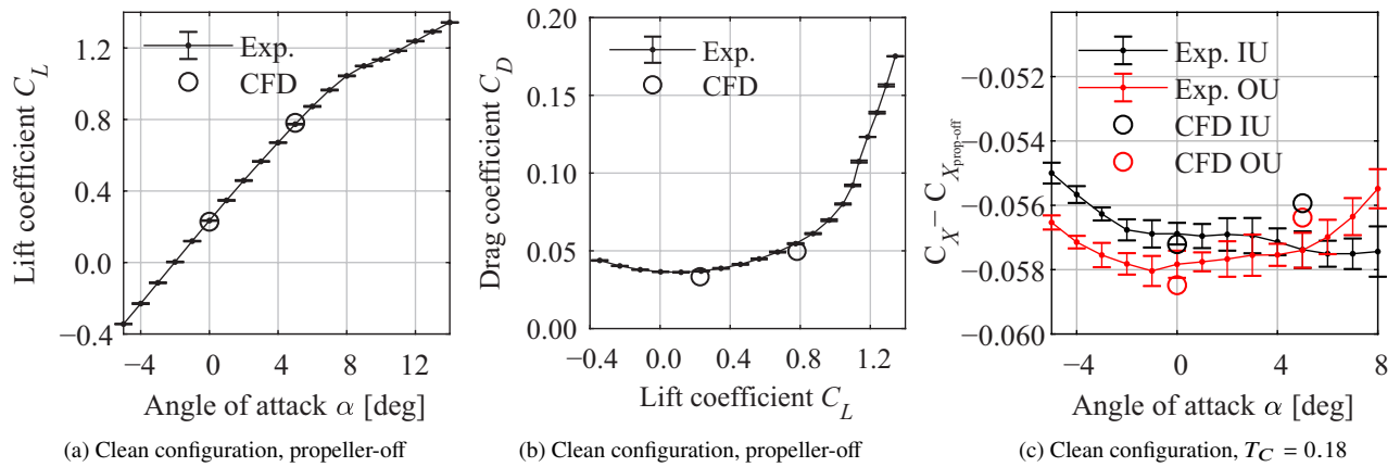
Fig. 7 Measured force coefficients compared with CFD.
