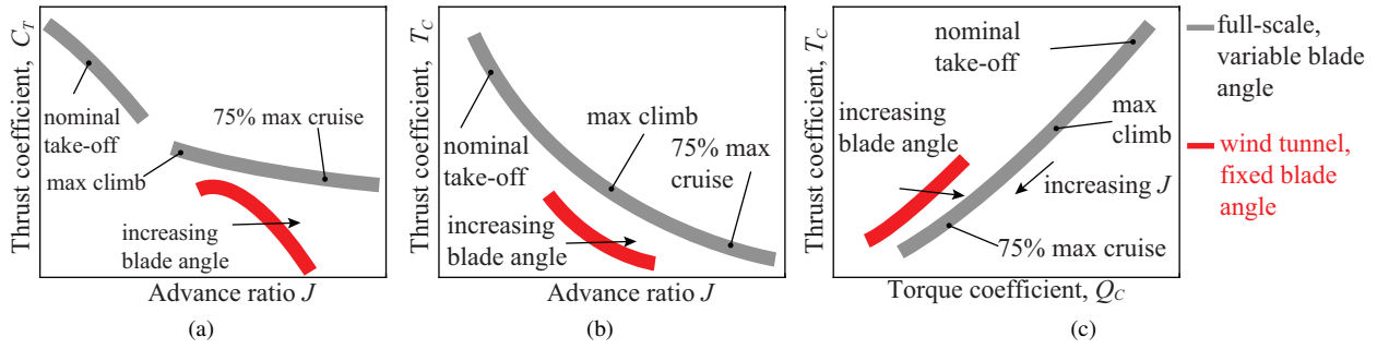
Fig. 4 Illustration of typical operating conditions for full-scale vs. wind-tunnel scale propellers. The red curve represents approximately the operating conditions in this paper.
