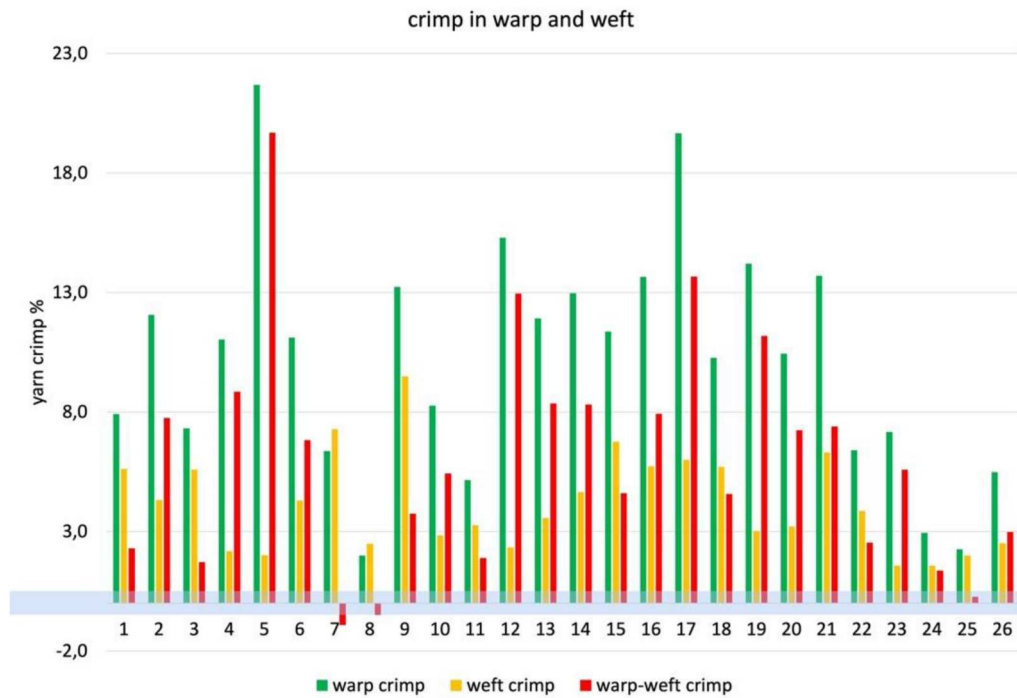
Figure 11. Crimp values in the warp are higher than in the weft in 96% of the cases.
