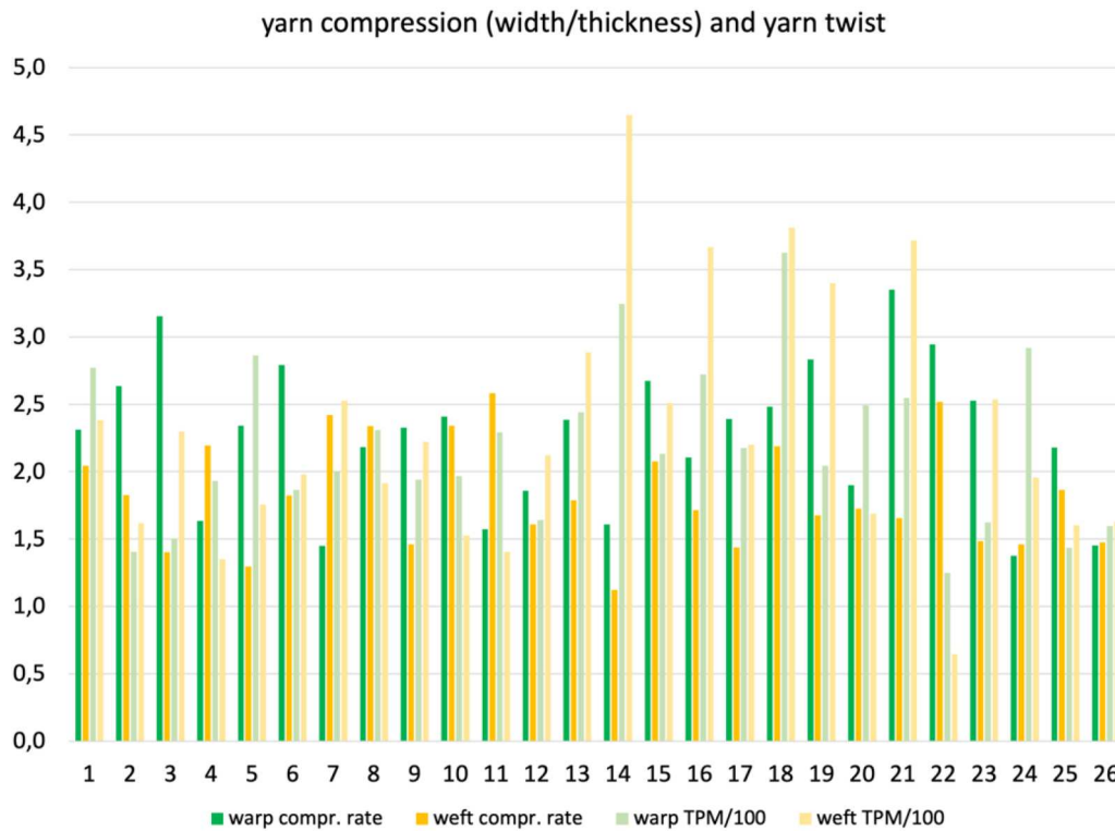
Figure 10. The yarn compression on the z axis of the textile (yarn width over thickness) and TPM. Higher TPM implies lower yarn compression.
