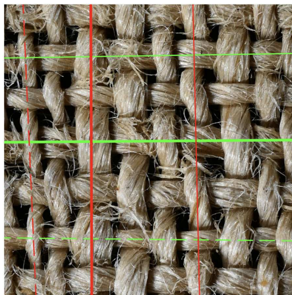
Figure 3. Example of the observations on the subsets. Yarns in warp (red) and weft (green) visually chosen to represent the small-medium-large subsets in the 1 cm 2 sample.
