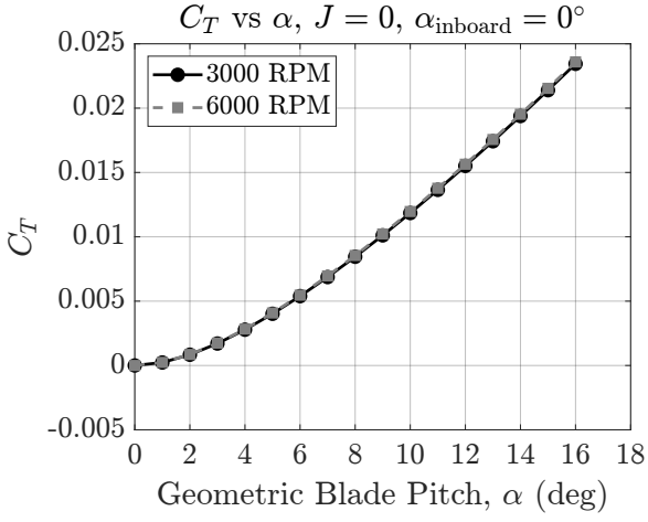
(a) C_T vs. \alpha at J = 0
