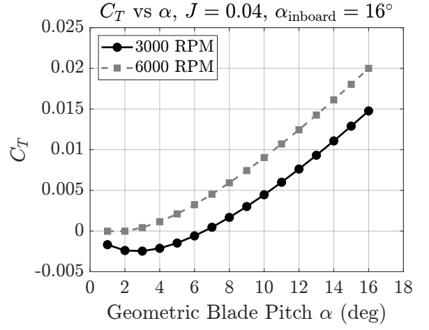
(b) C_T vs. \alpha at J = 0.04
