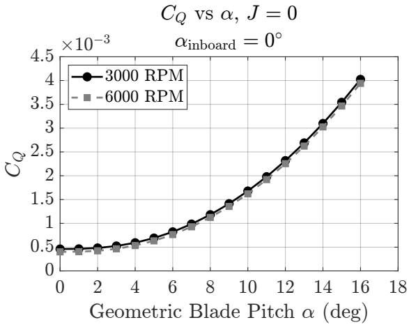
(c) C_Q vs. \alpha at J = 0
