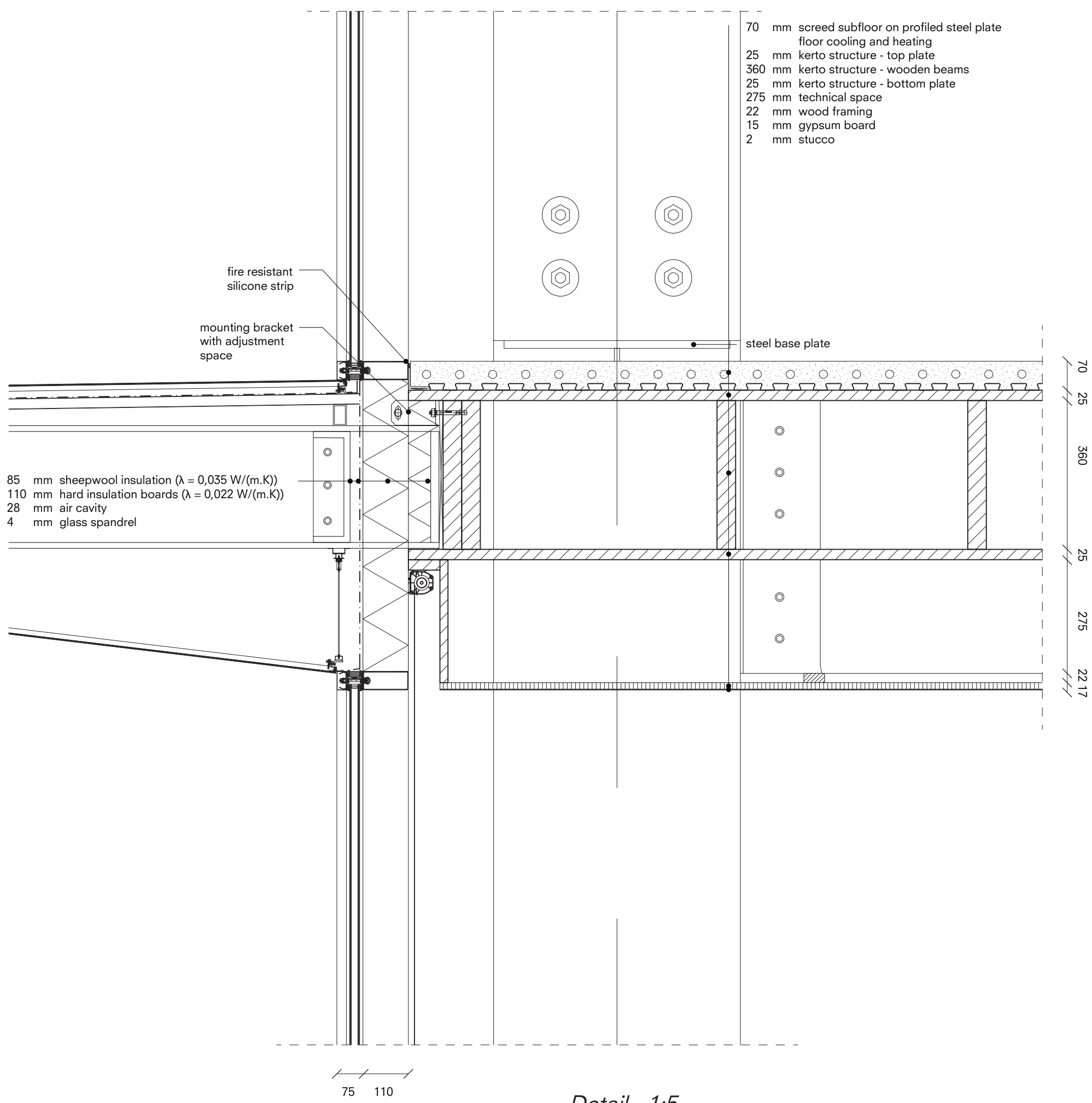
Detail - 1:5
