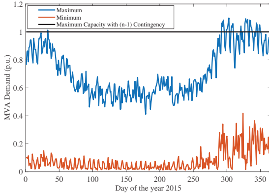
Fig. 4: Maximum and minimum daily MVA Demand from the critical medium voltage link in the year 2015 (data provided by Alliander).
