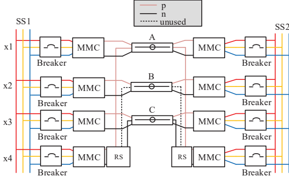
Fig. 6: Schematic for proposed topology 2.
