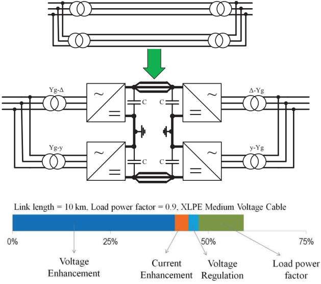
Fig. 2: Sample result for capacity enhancement due to various contributing factors by refurbishing underground double circuit ac cable link to operate under dc conditions (Proposed Topology 0) [3].
