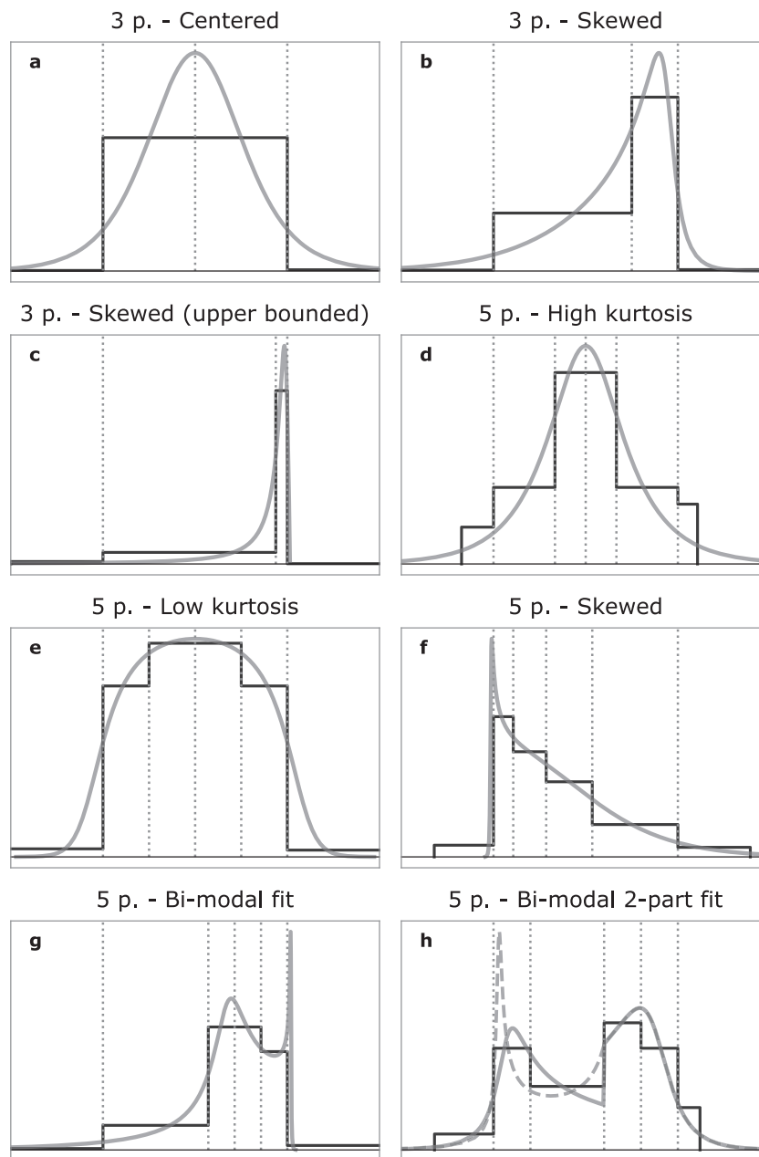
FIGURE 3 | 8 examples of Metalog distributions and piecewise uniform distributions fitted to 3-percentile (a–c) and 5-percentile (d–h) expert estimates. The estimates are indicated with the vertical dashed lines.
