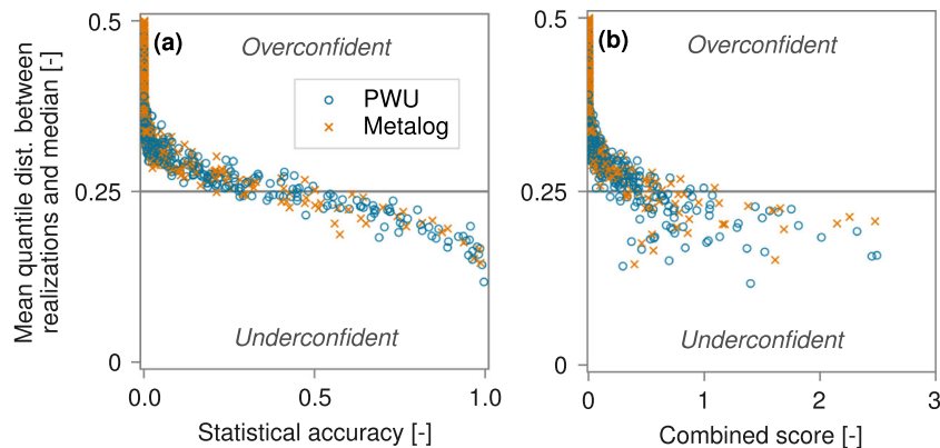
FIGURE 9 | Mean absolute difference between realization's quantile and median for CRPS. Plotted against statistical accuracy (a), and plotted against combined score (b).
