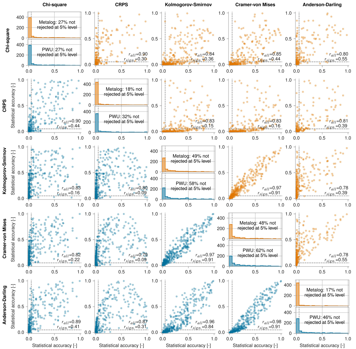
FIGURE 5 | Statistical accuracy for the 530 experts based on their quantile assessments in 49 case studies, using the Metalog distribution (upper right panels) and piecewise uniform (lower left panels). The dashed line represents the 5% significance level. The two numbers in the lower right of each panel are the rank correlation between all experts (above), and the rank correlation between all experts with a greater than 0.05 SA in both tests (below). Diagonal plots present the histogram of each measure's statistical accuracy for all 530 experts (i.e., the marginal distribution of each SA measure). In each histogram, the percentage of experts with a > 5% significance level is reported.
