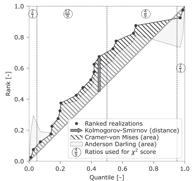
FIGURE 1 | Illustration of KS, CvM, and AD test statistics for a sample from a uniform distribution. The sample is plotted by their ranks (the connected dots). The arrow indicates the Kolmogorov-Smirnov (KS) statistic, the hatched area Cramer-von Mises (CvM), and the filled area (a weighted version of the hatched area) the Anderson-Darling (AD) statistic.
