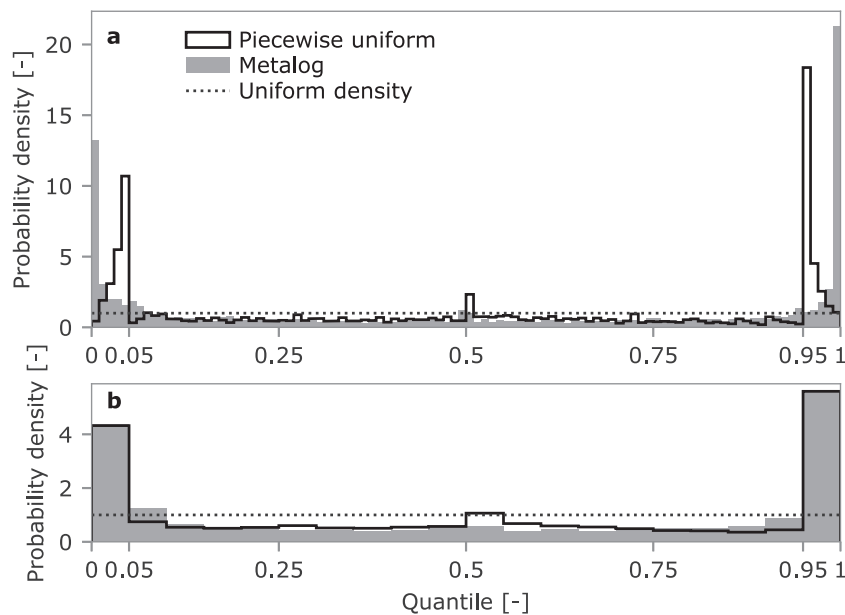
FIGURE 4 | Quantiles of realizations for 6864 individual expert quantile assessments with respect to the fitted piecewise uniform (white) and Metalog (grey) distributions. The difference between (a) with 100 bins and (b) with 20 bins shows the effect of assuming PWU or Metalog on the tail quantiles.
