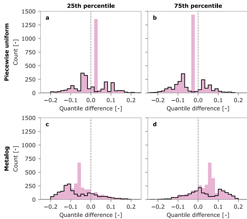
FIGURE 8 | Difference between the experts' estimated 25th percentile (a, c) and 75th percentile (b, d), and the positions according to the PWU distribution (a, b) and Metalog distribution (c, d) fitted to the five-percentile cases with the 25th and 75th percentile removed.
