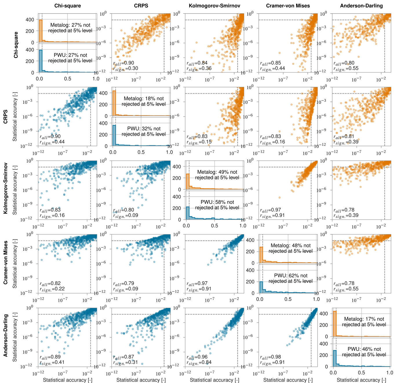
FIGURE A3 | Statistical accuracies for the 530 experts based on their quantile assessments in 49 case studies, using the Metalog distribution (upper right panel) and piecewise uniform (lower left panels). Similar to Figure 5 but on a logarithmic scale. The axes are limited to 10^{-12} , not showing SA values below this limit. The two numbers in the lower left of each panel are the rank correlation between all experts, and the rank correlation between all experts with a greater than 0.05 SA in both test. Diagonal plots present the histogram of each measure's statistical accuracy for all 530 experts (i.e., the marginal of each scatter plot). In each histogram, the percentage of experts with a > 5\% significance level is reported.
