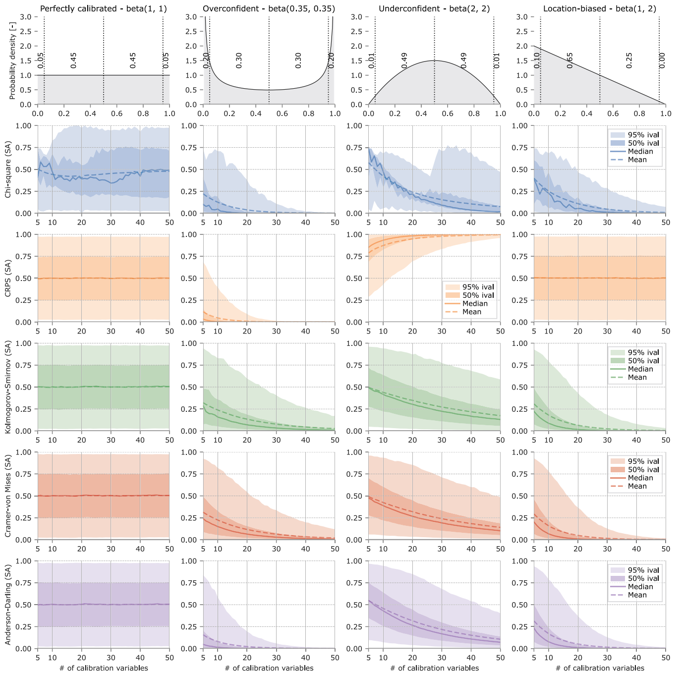
FIGURE 7 | Distribution of the DM's statistical accuracy for the different measures of statistical accuracy, resulting from drawing 10,000 samples of 5 up to 50 realization quantiles with different biases and evaluating their statistical accuracy. The four (non-)biases are: perfectly calibrated, overconfident, underconfident, and location-biased (overestimating).
