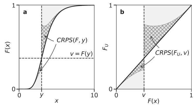
FIGURE 2 | Illustration of regular CRPS (a) and scale invariant CRPS (b). The CRPS is calculated by summing the squared difference between the CDF and step function, which is illustrated with the crossed area.
