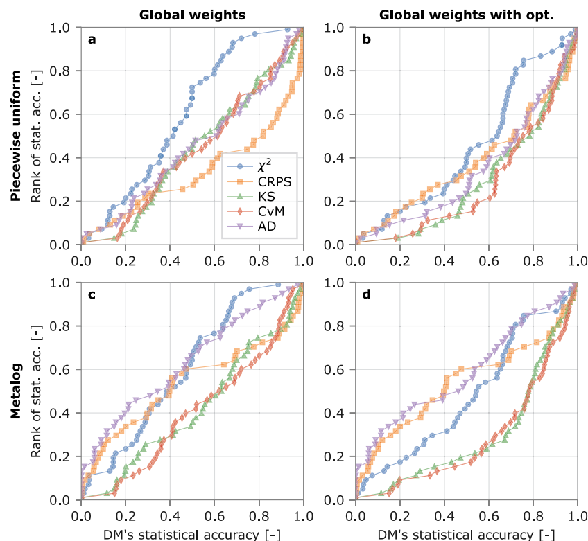
FIGURE A1 | Empirical distributions of the decision makers' statistical accuracies in the 49 case-studies. (a) and (b) for piecewise uniform distribution, (c) and (d) for the Metalog; (a) and (c) for the global weights DM without optimization, and (b) and (d) with optimization.
