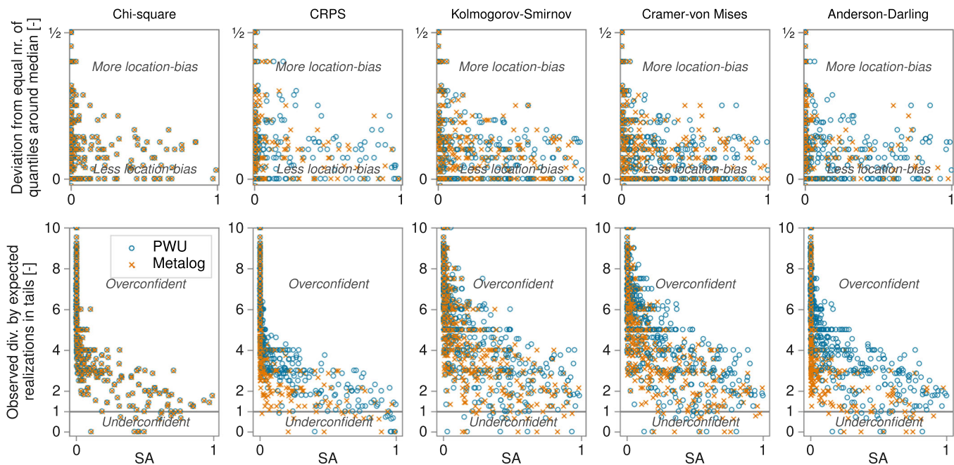
FIGURE 6 | Sensitivity of the measures of statistical accuracy to biases. The top row shows sensitivity to under- and overestimating experts (location-bias), calculated using Eq. 6. The bottom row shows under- and overconfidence, calculated using Eq. 7. Orange crosses indicate statistical accuracy calculated for the Metalog, blue circles for the piecewise uniform distribution.
